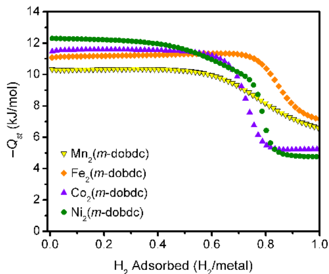
Figure 3. H_2 isosteric heat of adsorption curves for the M_2(m\text{-dobdc}) series of frameworks, as a function of the amount adsorbed.
