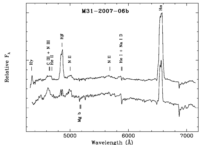
FIG. 3.—Follow-up spectra of M31N-2007-06b taken with the LRS on the HET ( upper spectrum : \sim 1 week after eruption; lower spectrum : \sim 5 weeks after eruption). As the nova faded, note the increasing contamination by light from the globular cluster Bol 111, resulting in Balmer and Mg b absorption features.
