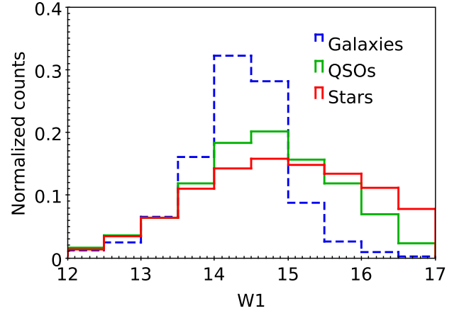
Fig. 2. Normalised number counts of W1 magnitudes in the WISE \times SCOS \times SDSS cross-matched sample for stars, galaxies, and quasars.
