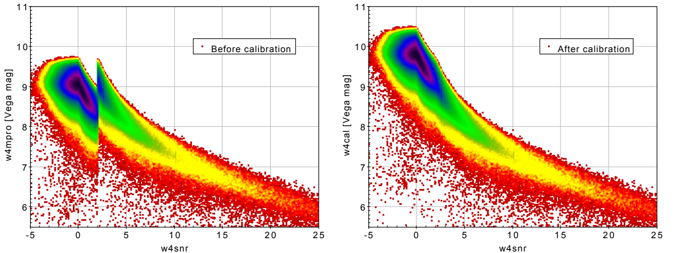
Fig. A.2. Illustration of the calibration procedure of W4 upper limits and non-detections: values from the database ( left panel ) and after our empirical offset by +0.75 mag for the w4\text{snr} < 2 sources ( right panel ).
