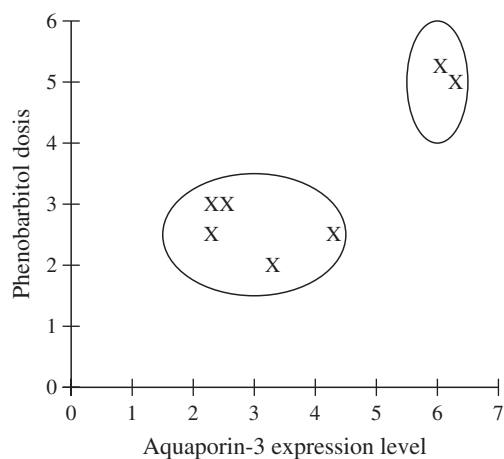
Figure 8: Partition clustering.
