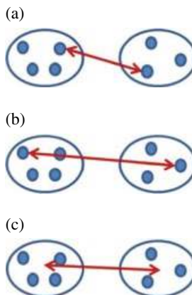
FIGURE 18 Agglomerative HCA cluster dissimilarities: (a) single linkage, (b) complete linkage, and (c) group average.
