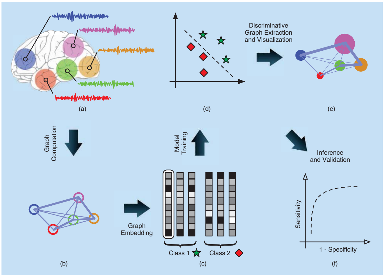
[FIG1] Overall scheme for predictive modeling with brain graphs. (a) Imaging data are first preprocessed, then the brain is divided into regions, and each region is assigned a regional representative time series. (b) A labeled simple graph is computed from the regional time series, where edge labels correspond to statistical dependency between brain regions, and brain regions are mapped to graph vertices. (c) The graph is embedded into a vector space, after which (d) statistical machine learning can be used. (e) Brain-space visualization of the discriminative pattern used by the classifier is critical for interpretation. (f) Statistics and confidence intervals can be obtained on inference results, allowing validation of the techniques when used, e.g., to elicit imaging markers in clinical applications.
