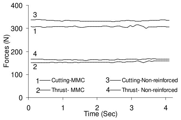
(b) feed 0.4 mm/rev and speed 400 m/min
