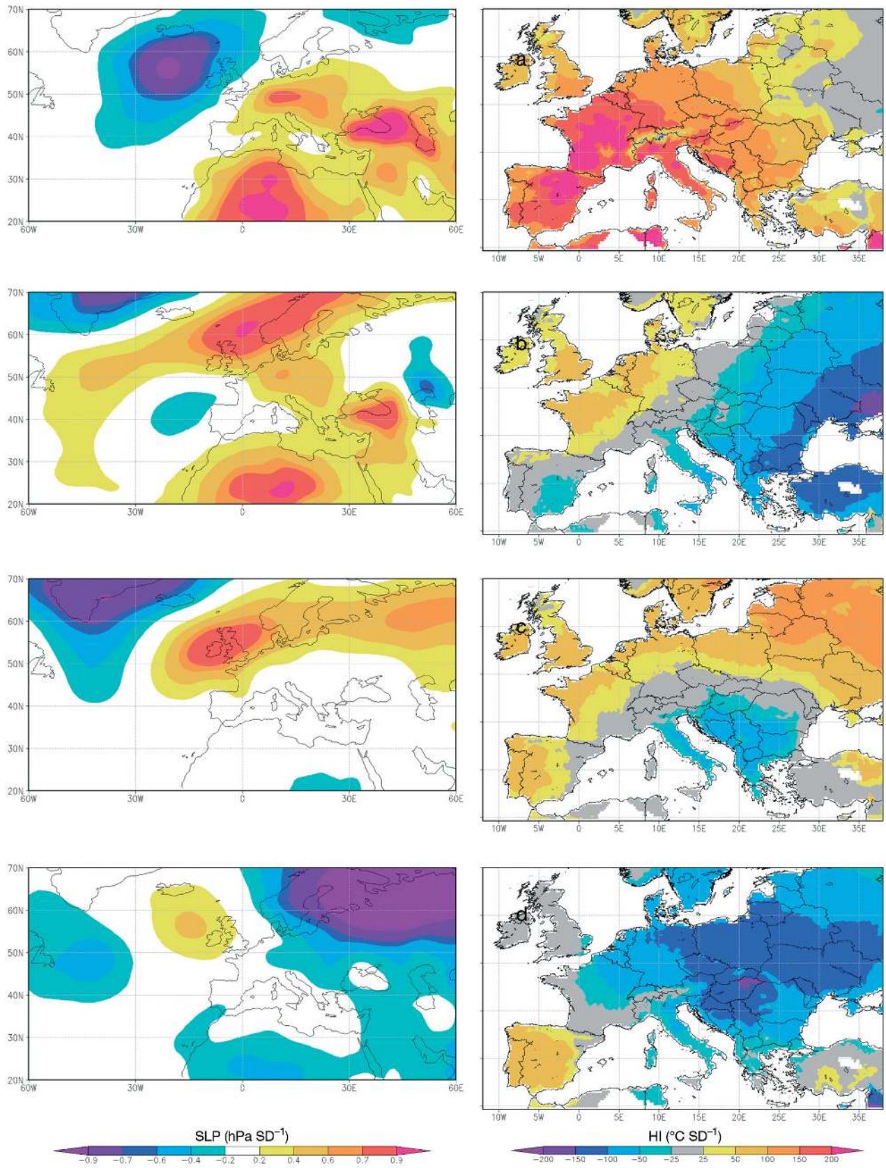
Fig. 8. The same as described in Fig. 7, but for the mean sea level pressure (SLP, left panels). Canonical correlations are 0.82, 0.61, 0.60 and 0.44 (statistically significant at 95% confidence level; Bartlett-Lawley test)
