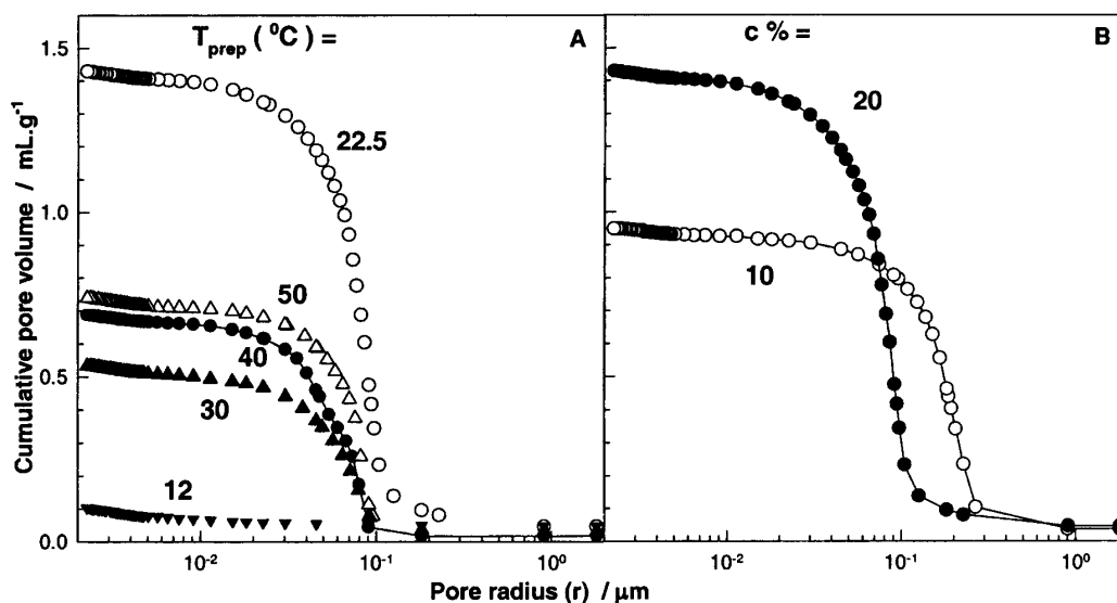
Figure 2. Integral size distributions of the pores in PNIPA networks. (A): c = 20 w/v %. (B): T_{prep} = 22.5^{\circ}\text{C} . Synthesis variables are indicated in the Figures.
