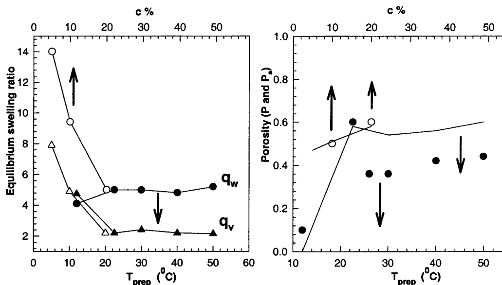
Figure 4 (left): Equilibrium weight ( q_w ) and volume swelling ratios ( q_v ) of the networks shown as function of the gel preparation temperature T_{prep} (filled symbols) and the initial monomer concentration c (open symbols). Circles and triangles represent the q_w and q_v values, respectively. Figure 5 (right): Total porosities of the networks P shown as function of the gel preparation temperature T_{prep} (filled symbols) and the initial monomer concentration c (open symbols). The lines were calculated using eq. (4) and they represent the swollen state porosities P_s .
