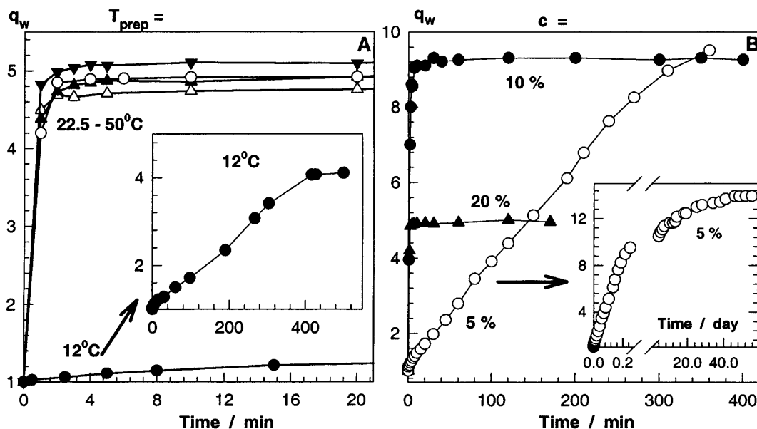
Figure 1. Weight swelling ratio q_w of PNIPA networks in water at 20°C shown as a function of the swelling time. (A): c = 20 w/v %, T_{prep} = 12 (●), 22.5 (■), 30 (▲), 40 (○), and 50°C (○). (B): T_{prep} = 22.5 °C. The initial monomer concentrations c are indicated in the figure.
