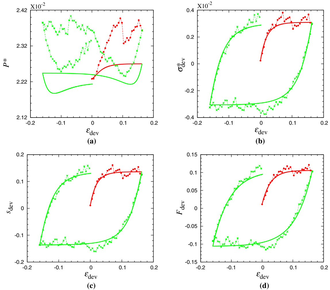
Fig. 14 Evolution of a pressure P^* , b deviatoric (shear) stress \sigma_{dev}^* , c normalized shear stress s_{dev} , and d deviatoric fabric F_{dev} with shear strain \epsilon_{dev} during cyclic shear at constant volume \nu = 0.711 , starting from an initial isotropic configuration. The values of s_{dev}^{max} , F_{dev}^{max} and \beta_F for \nu = 0.711 are 0.167, 0.124 and 40.04, respectively, taken directly from the relations proposed in Refs. [30,39]. The red circle data points are the DEM simulation data over which the calibration of moduli was done, while the green asterisk data points represent unloading (reversal) and re-loading. The solid line is the prediction of the DEM observations using Eq. (18) (color figure online)
