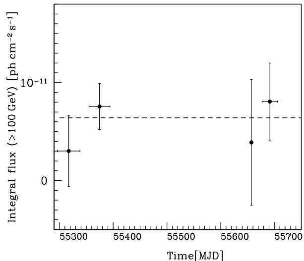
Figure 4. 1ES 1741+196 light curve during MAGIC observation period in a time bin of 28 days. The horizontal line represents the fit to the data assuming a constant flux (see text for details).
