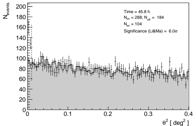
Figure 3. \theta^2 distributions of the 1ES 1741+196 signal and background estimation from 46 hr of MAGIC stereo observations for E > 250 GeV. The region between zero and the vertical dashed line (at 0.01 degrees 2 ) represents the signal region.
