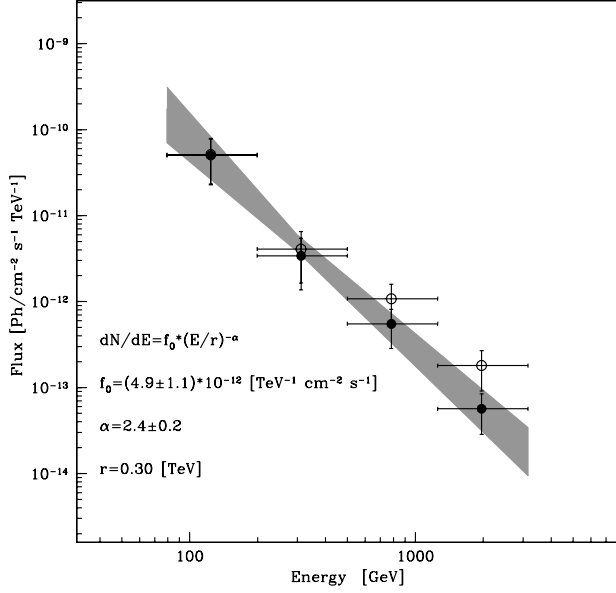
Figure 5. 1ES 1741+196 differential energy spectrum measured by MAGIC (filled circle), and EBL corrected spectrum using the Franceschini et al. (2008) model (empty circle). The fit function is shown as a grey bow-tie.
