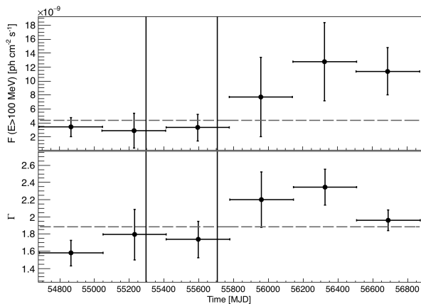
Figure 2. 1-year binning Fermi /LAT light curve for E > 100 MeV (top) and evolution of the spectral index as a function of the time (bottom). The grey dashed lines represent the mean flux and spectral index during the first 6.7 years of the mission, respectively. The period between the vertical bars denotes the MAGIC observation window.
