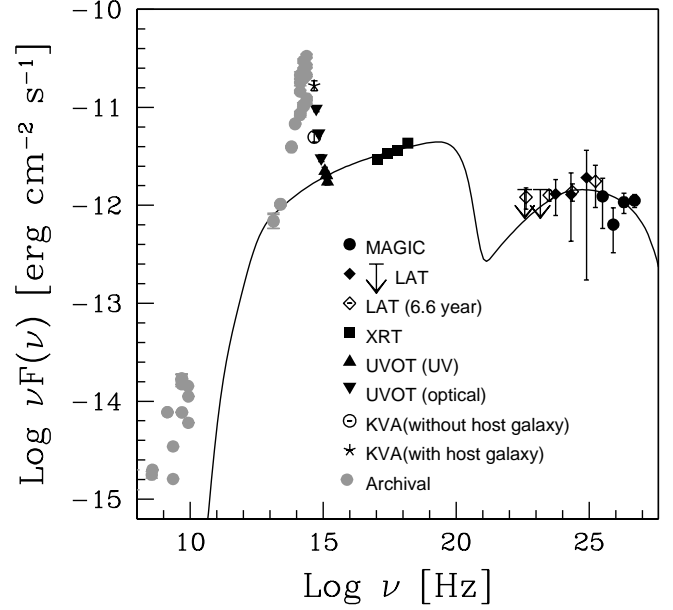
Figure 6. The SED of 1ES 1741+196 from eV to TeV energies. The UV (UVOT UVW1, UVM2, UVW2: filled triangle) fluxes attributed to the nuclear region of blazar are used for the SED fitting – whereas the optical fluxes (KVA: empty circle; UVOT V, B, U: filled inverted triangle) are not. The UVOT UV fluxes are corrected for both the Galactic extinction and the host galaxy, while UVOT optical fluxes are corrected only for the former. The KVA flux with (empty circle) and without (star) subtracting the host galaxy magnitude are also shown. X-ray data (filled square) come from Swift /XRT, averaged over two distinct observations. Contemporaneous (filled diamond) and 6.6-yr-integrated (empty diamond; for comparison) HE \gamma -ray data come from Fermi /LAT. MAGIC data (filled circle) are EBL corrected (Franceschini et al. 2008). We also show the archival data (filled gray circle) for comparison.
