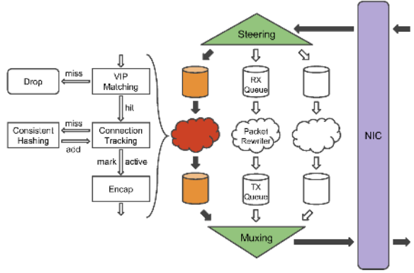
Figure 4: Maglev forwarder structure.
