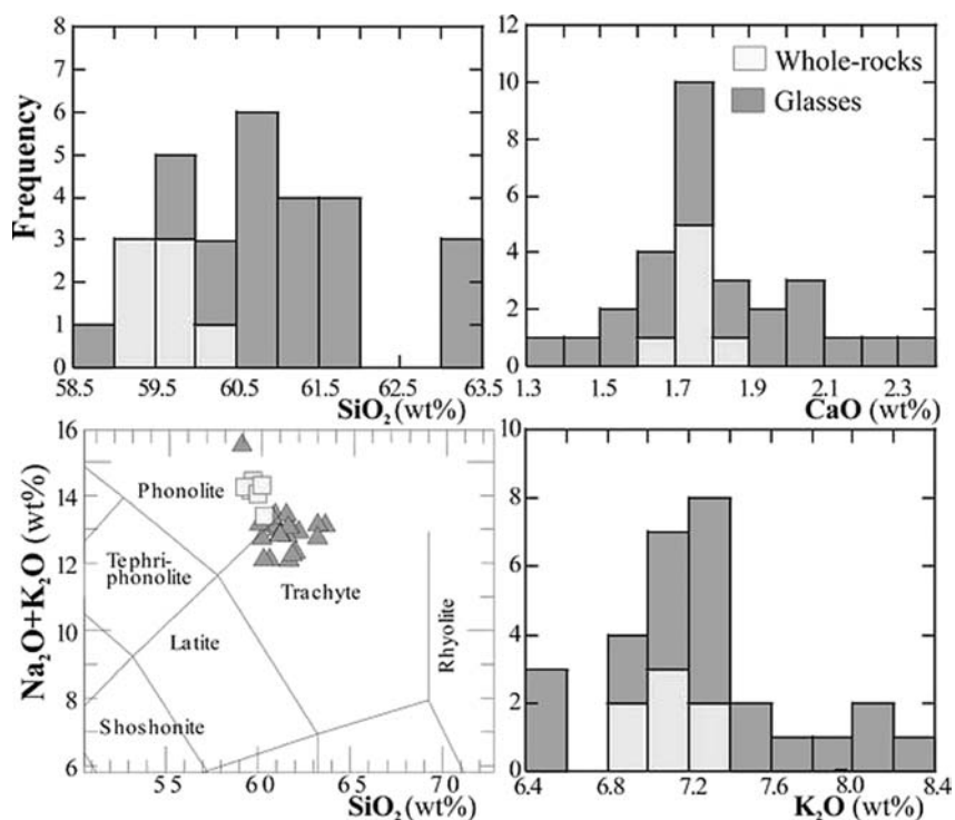
Fig. 3 Compositional diagrams for Monte Nuovo glass matrix. Whole-rocks compositions from Rosi and Sbrana (1987) are reported for comparison
