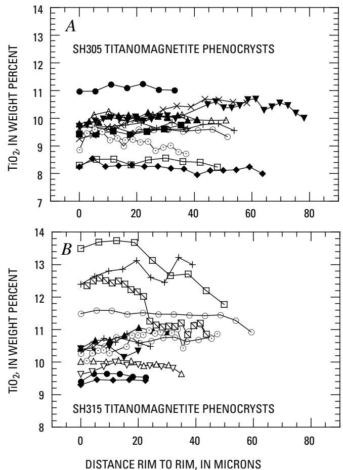
Figure 9. Composition ( \text{TiO}_2 ) profiles across representative titanomagnetite phenocrysts in samples SH305 (A) and SH315 (B) from the 2004–6 eruption, showing range of relatively homogeneous crystals present.
