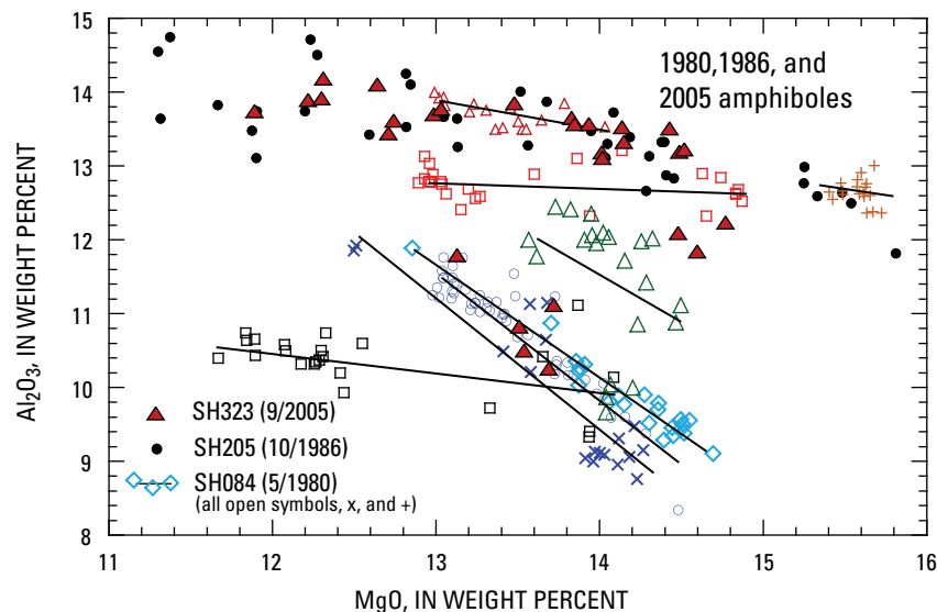
Figure 14. Compositions of eight amphibole phenocrysts (rim to rim transects) in the 1980 Mount St. Helens pumice (SH084) compared with similar amphibole transects for a typical sample of the 2004–6 lava dome (SH323) and 1986 dome (SH205). Lines are fit to the eight SH084 amphibole profiles. Zoning in the 1980 pumice phenocrysts is similar to that in the 2004–6 phenocrysts except that it occurs at lower \text{Al}_2\text{O}_3 in most crystals. Note that rims on SH323 amphiboles spread over the low- \text{Al}_2\text{O}_3 compositions found in the May 1980 samples, whereas the zoning profile in SH205 (1986 lava) is indistinguishable from 2004–6 samples such as SH304 and SH305 (fig. 4).
