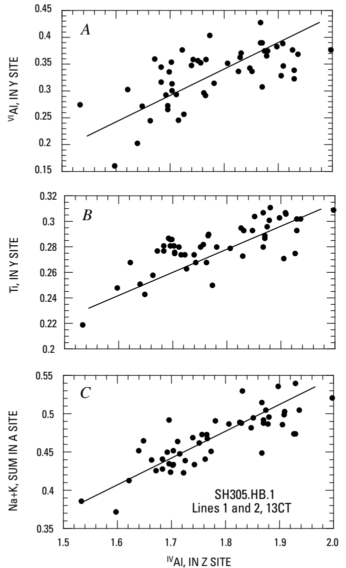
Figure 5. Plots showing position of chemical species in crystallographic sites versus tetrahedrally coordinated Al ( IV Al) in Z site for typical, cyclically zoned amphibole in lava samples from Mount St. Helens 2004–6 eruption. A , Octahedrally coordinated Al ( VI Al) in the Y site. B , Ti in the Y site. C , Sum of Na+K in the A site. Note that approximately equal amounts of the IV Al increase are balanced by increases in VI Al and the sum of Na and K.
