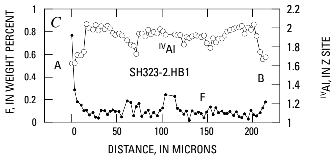
Figure 7. Typical amphibole phenocryst in sample SH323 erupted in September 2005 when the mass eruption rate had dropped to about 1\ \text{m}^3/\text{s} (Pallister and others, this volume, chap. 30). A , Backscattered electron image showing compositional traverse as line A–B. B , C , Compositional traverses, showing presence of a rim less than 30\ \mu\text{m} thick with low Al and Mg (panel B ) and high F (panel C ). Profile for \text{SiO}_2 across same phenocryst (fig. 4) shows the rim is also enriched in Si.
