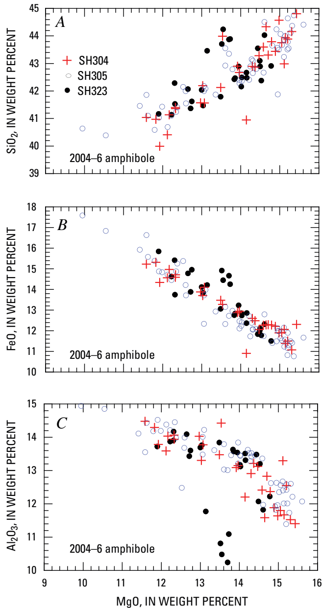
Figure 4. Chemical variation diagrams showing rim-to-rim compositional zoning in typical amphibole phenocrysts from three samples of the 2004–6 eruption. A , MgO vs. SiO 2 . B , MgO vs. FeO. C , MgO vs. Al 2 O 3 . Crystal rims in SH323 (five points) with anomalously high SiO 2 (panel A ) and low Al 2 O 3 (panel C ) are discussed elsewhere in the paper.
