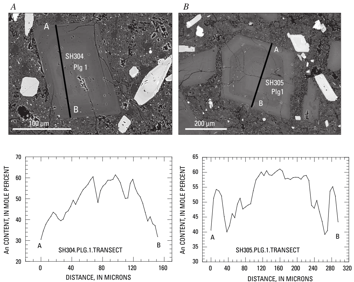
Figure 2. Backscattered electron images from thin section of Mount St. Helens lava, showing typical plagioclase phenocryst of 2004–6 lava. Images show cycles of light (Ca-rich) and dark (Na-rich) phenocryst growth; accompanying graphs depict An concentrations along the A–B profiles. A, Plagioclase in sample SH304. B, Plagioclase in sample SH305.
