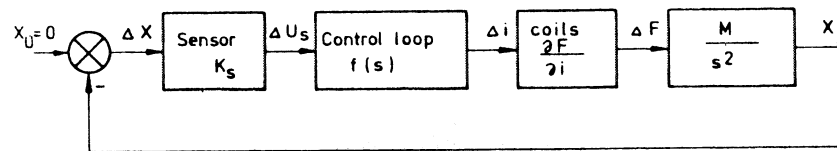
Figure 4: Translational Control Loop
