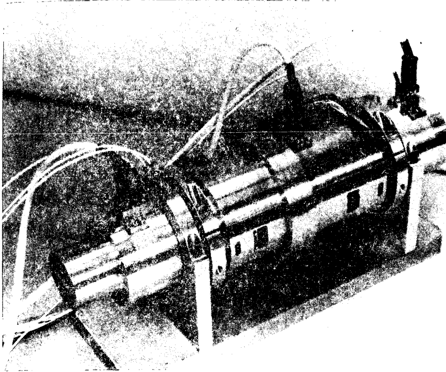
Figure 1. Photograph, Magnetically Suspended Motor Rotor
