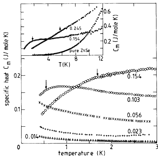
FIG. 4. Magnetic specific heat of Zn_{1-x}Mn_xSe [ x=0.014 ( \Delta ), 0.023 ( + ), 0.056 ( x ), 0.103 ( \circ ), and 0.154 ( \diamond )]. Inset: magnetic specific heat of Zn_{1-x}Mn_xSe ( x=0.154 and 0.245 as well as specific heat of pure ZnSe). The arrows indicate the freezing temperatures T_f .
