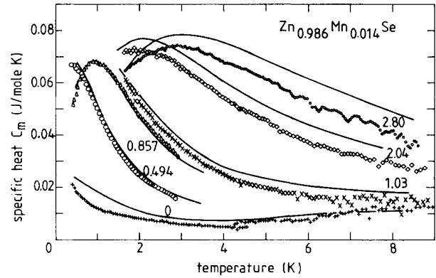
FIG. 5. Magnetic field dependence of the magnetic specific heat of Zn_{0.986}Mn_{0.014}Se for B=0.00, 0.494, 0.857, 1.03, 2.04, and 2.80 T. The solid lines are obtained from the ENNPA using J_0/k_B = -13 K and J_1/k_B = -7/R K. 6,8
