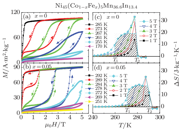
Fig. 18. Magnetization isotherms for \text{Ni}_{45}(\text{Co}_{1-x}\text{Fe}_x)_5\text{Mn}_{36.6}\text{In}_{13.4} ((a) x = 0 and (b) x = 0.05 ), and the magnetic entropy change \Delta S as a function of temperature under different magnetic fields for (c) x = 0 and (d) x = 0.05 . The shadow area indicates the direct RC evaluated by integrating the area under the \Delta S curve from T_1 to T_2 ( T_2 - T_1 : half-maximum width). Arrows indicate field changing paths. [53]
