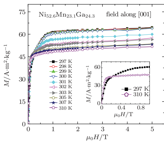
Fig. 4. Isothermal M-H curves with magnetic field along the [001] direction at different temperatures for single crystal \text{Ni}_{52.6}\text{Mn}_{23.1}\text{Ga}_{24.3} . The inset displays the detailed M-H curves at 297 K and 310 K. [12]
