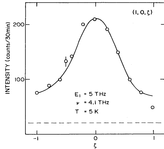
FIG. 11. Constant-frequency scan at 4.1 THz in the ordered phase of URu_2Si_2 through the antiferromagnetic zone center at (1,0,0) . The data were obtained with configuration No. 5 of Table I. The dashed line is the background measured with analyzer turned. The solid line is a guide to the eye.
