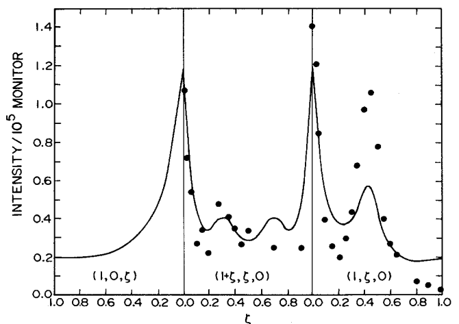
FIG. 7. Wave-vector dependence of the integrated spin-wave intensity divided by the polarization factor (1 - q_z^2) for \text{URu}_2\text{Si}_2 .
