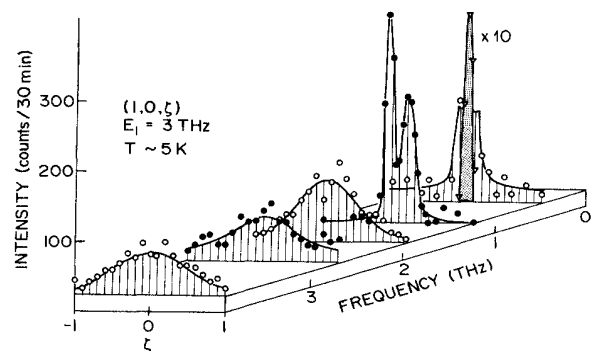
FIG. 12. Perspective view of the scattered neutron intensity vs energy transfer and momentum transfer along (1,0,\xi) . The data are taken in the ordered phase at T=5 K. The asymmetry in the double-peak structure is due to a resolution effect. The solid lines are guides to the eye. Solid and open symbols are used for clarity of presentation. At \nu=0.5 THz the data plotted as triangles which define the hatched region has been reduced by a factor 10.
