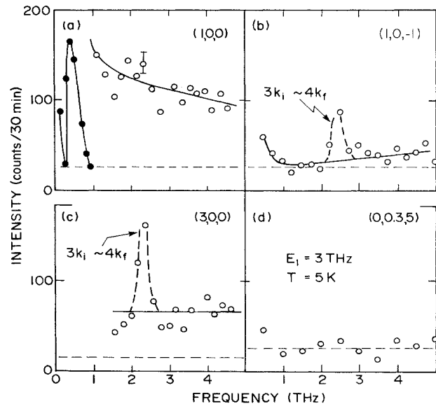
FIG. 10. Low-temperature energy scans at four different reciprocal lattice points taken with configuration No. 4 of Table I. Solid points in (a) are reduced by a factor of 10. The lines through the data are guides to the eye. The dashed line is the background as measured with the analyzer turned away from reflection. The peaks in (b) and (c) arise from a spurious process involving third-order neutrons.
