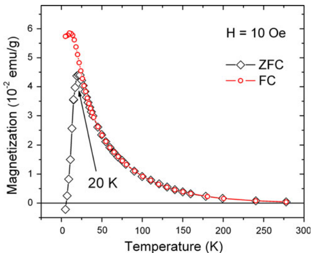
Fig. 9 Zero-field-cooled and field-cooled magnetization as a function of temperature for Fe doped ZnO nanofibers
