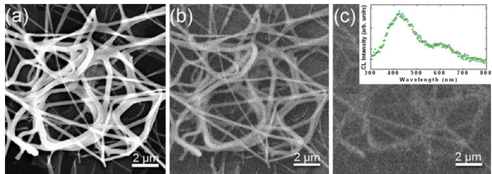
Fig. 6 SEM (a), CL panchromatic (b) and CL at 400 nm (c) images of Fe doped ZnO nanofibers. Inset: CL spectrum Fe doped nanofibers
