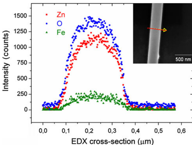
Fig. 5 The EDX signal for Zn, O and Fe atoms across Fe doped ZnO nanofiber. Homogeneous distribution of Fe atoms is proved
