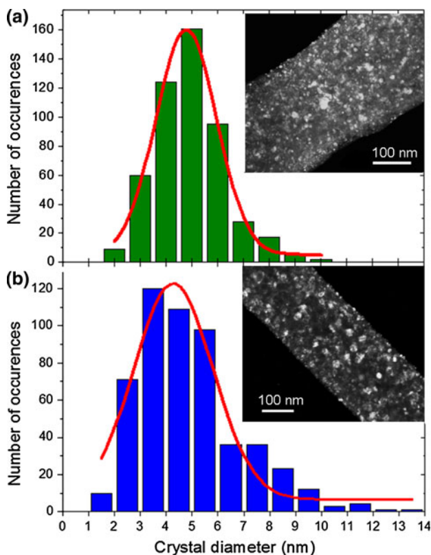
Fig. 4 Crystal size distribution of: Fe doped (a) and undoped ZnO nanofibers (b) obtained from the TEM measurements. The dark field images: Fe doped (a) and undoped (b) ZnO nanofibers, respectively (inset)
