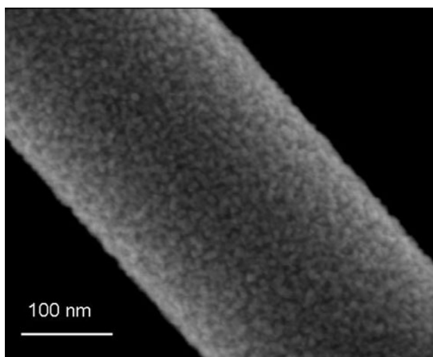
Fig. 1 SEM image of the Fe doped ZnO nanofiber showing that it is formed by the conglomerates of nanocrystallites few nanometer in diameter
