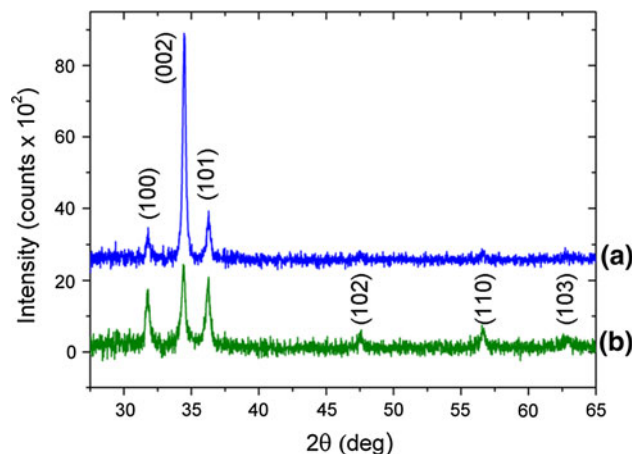
Fig. 2 XRD patterns of ZnO nanofibers: undoped (a) and Fe doped (b). The top spectrum is shifted by 2,500 counts for clarity
