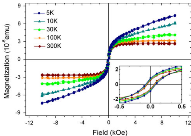
Fig. 7 Effect of magnetization on magnetic field of Fe doped ZnO nanofibers oriented along the applied magnetic field in the magnetometer for various temperatures. Enlargement of the hysteresis loops in the -0.5 to 0.5 kOe magnetic field range ( inset )
