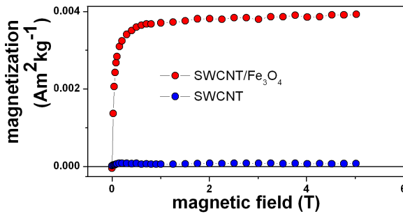
Fig. 2. Magnetic properties of the samples with volume concentration of magnetic nanoparticles \Phi = 2 \times 10^{-3} measured at room temperature.
