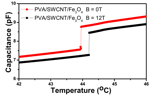
Fig. 3. The temperature dependence of capacitance of the samples with volume concentration of magnetic nanoparticles \Phi = 2 \times 10^{-3} measured without magnetic field and in magnetic field 12 T.
