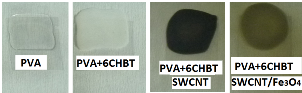
Fig. 1. The photo of the prepared samples.
