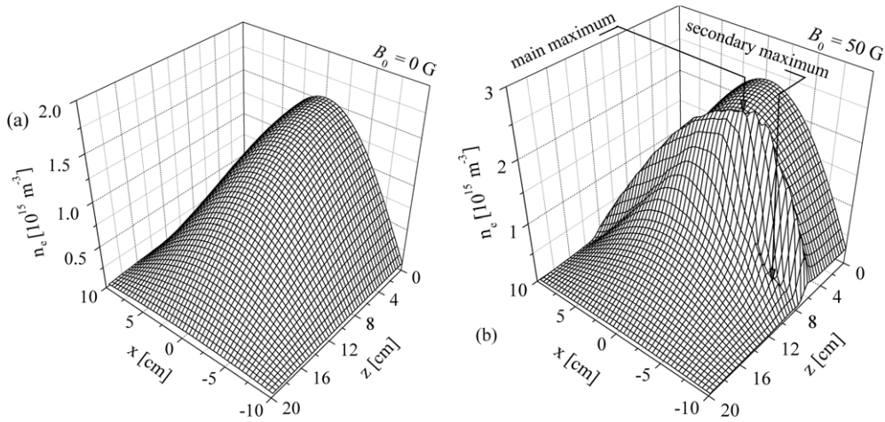
Figure 4. Spatial distribution of the electron concentration obtained within the 2D-model for B_0 = 0 G (a) and B_0 = 50 G (b).
