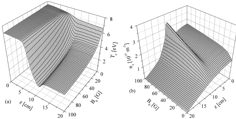
Figure 7. Changes in the axial distribution, for x = 0 , of the electron temperature (a) and the density (b) for varying values of the magnetic field B_0 obtained from the 2D-model.
