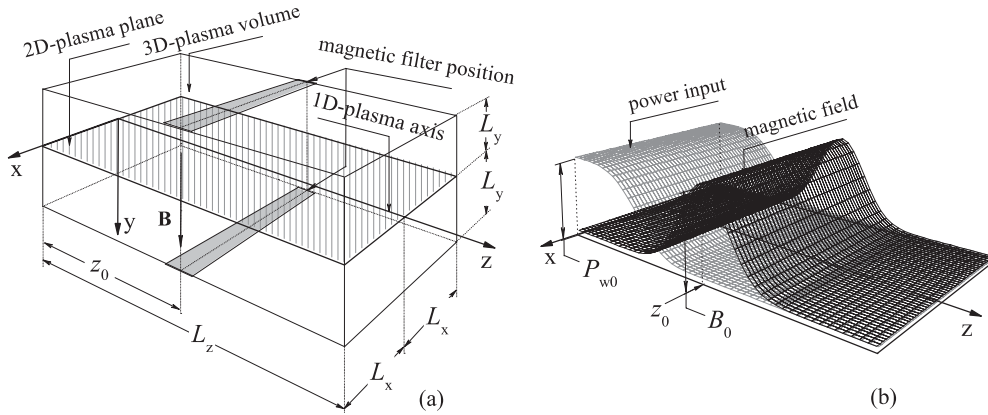
Figure 1. Configuration of the plasma volume in (a) and an illustration of the z -variations of the magnetic field and of the power input in (b).
