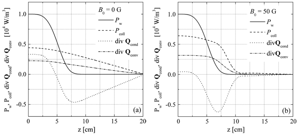
Figure 8. Axial changes, for x = 0 , of the different terms ( P_w , P_{\text{coll}} and the contributions of the conductive and convective fluxes to \text{div } \mathbf{Q}_e ) in the electron-energy balance (5) for B_0 = 0 \text{ G} (a) and B_0 = 50 \text{ G} (b); results from the 2D-model.
