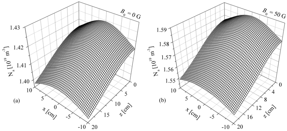
Figure 6. Spatial distribution of the atomic gas component obtained within the 2D-model for B_0 = 0 G (a) and B_0 = 50 G (b).
