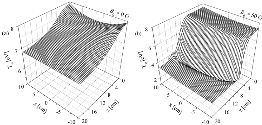
Figure 3. Spatial distribution of the electron temperature obtained within the 2D-model for B_0 = 0 G (a) and B_0 = 50 G (b).
