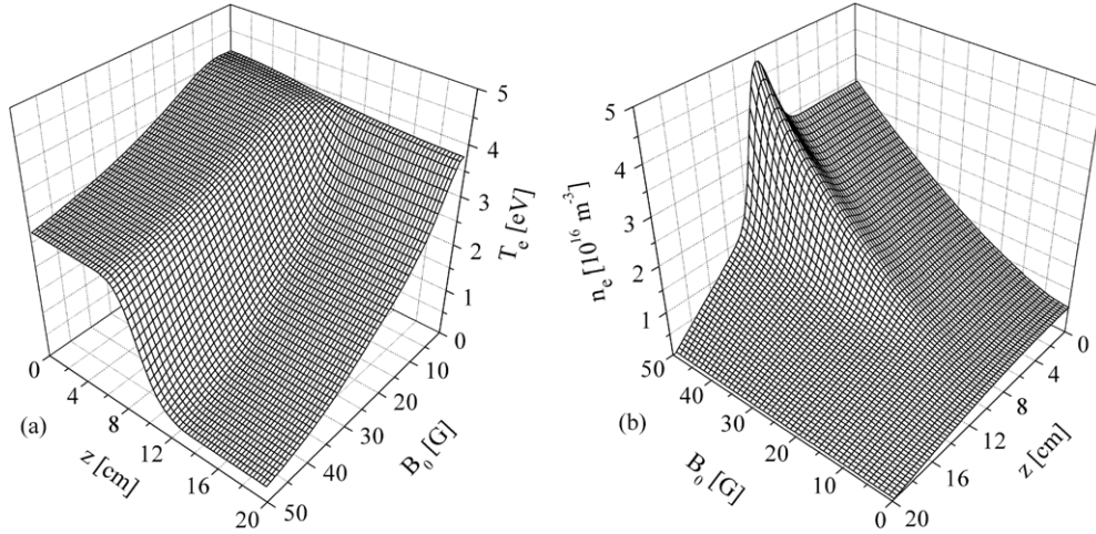
Figure 2. Results from the 1D-model: axial distribution of the electron temperature (a) and density (b) for varying values of the magnetic field B_0 at the centre of the filter.
