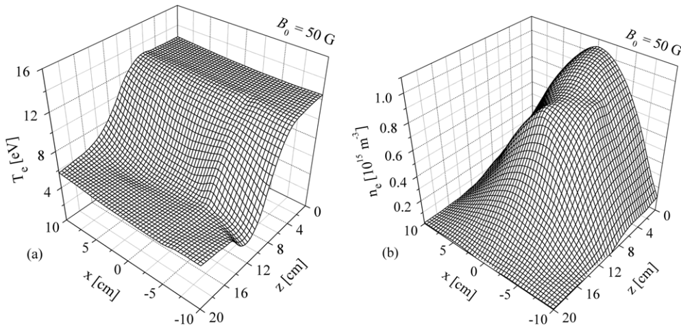
Figure 10. Results from the 3D-model: spatial distribution of the electron temperature (a) and the density (b) obtained in the (x-z) -plane, for y = 0 .
