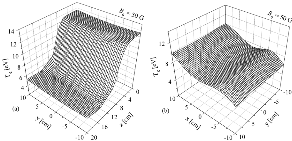
Figure 11. Results from the 3D-model: spatial distribution of the electron temperature in the (y-z) -plane for x = 0 in (a) and in the (x-y) -plane for z \equiv z_0 = 10 cm in (b).
