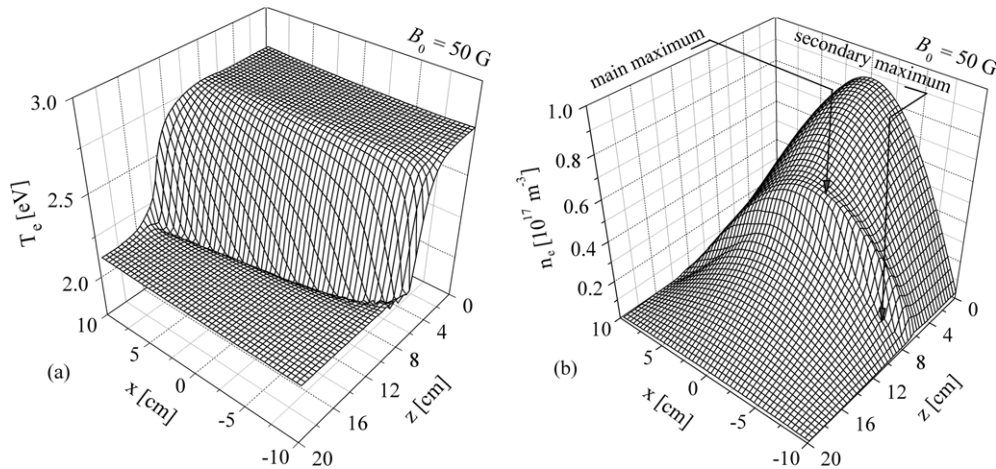
Figure 9. An argon discharge: spatial distribution of the electron temperature (a) and the density (b) obtained within the 2D-model.
