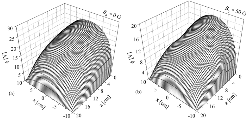
Figure 5. Spatial distribution of the potential of the dc electric field obtained within the 2D-model for B_0 = 0 G (a) and B_0 = 50 G (b).
