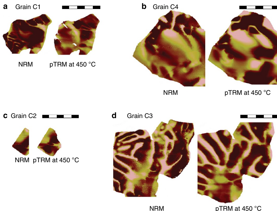
Figure 5 | Grains in the sample subjected to a pTRM at 450 °C. Again, the images of the grains in their NRM state on the left and the images of the grains in their pTRM state on the right. All scale bars are 5 μm. Changes are evident, as expected after heating the grains well above their alteration temperature, as indicated by the susceptibility-versus-temperature experiments (Supplementary Fig. 7). Domains tend to become larger in the pTRM state, and domain walls more distinct (b, d). This behaviour is most evident in the upper left-hand corner of grain C3 (d), where narrow NRM domains change their orientation by ~90°. The smaller grains, C1 and C2 (a and c, respectively), appear less affected by the alteration at high temperatures, better reproducing the NRM domain state than the larger grains. However, the curvy domain configurations as observed in the grains heated to 250 °C (Fig. 3), are not seen here.
