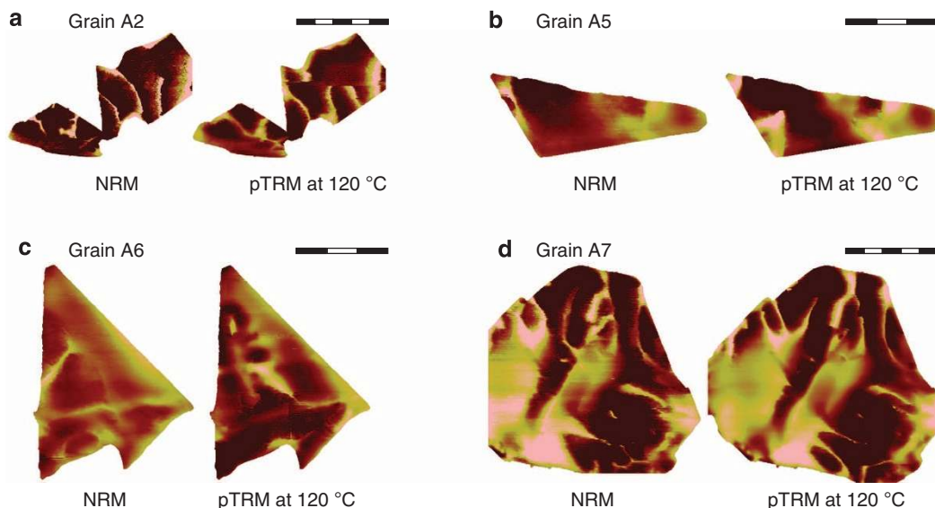
Figure 3 | Grains in the sample subjected to a pTRM at 120\ ^\circ\text{C} . ( a-d ) Four typical grains in their NRM state (left-hand side images) and pTRM state (right-hand side images). Domain structures hardly change; especially in grains A2 ( a ) and A7 ( d ) the configuration is remarkably similar in the pTRM state. Grains A5 ( b ) (in its lower left corner) and A6 ( c ) (in the centre) do show minor changes, however. The chemical analyses (Supplementary Table 1) indicate a relatively high Ti-content for these grains, lowering their Curie temperature. Scale bar, 5\ \mu\text{m} ( a,d ); 3\ \mu\text{m} ( b,c ).
