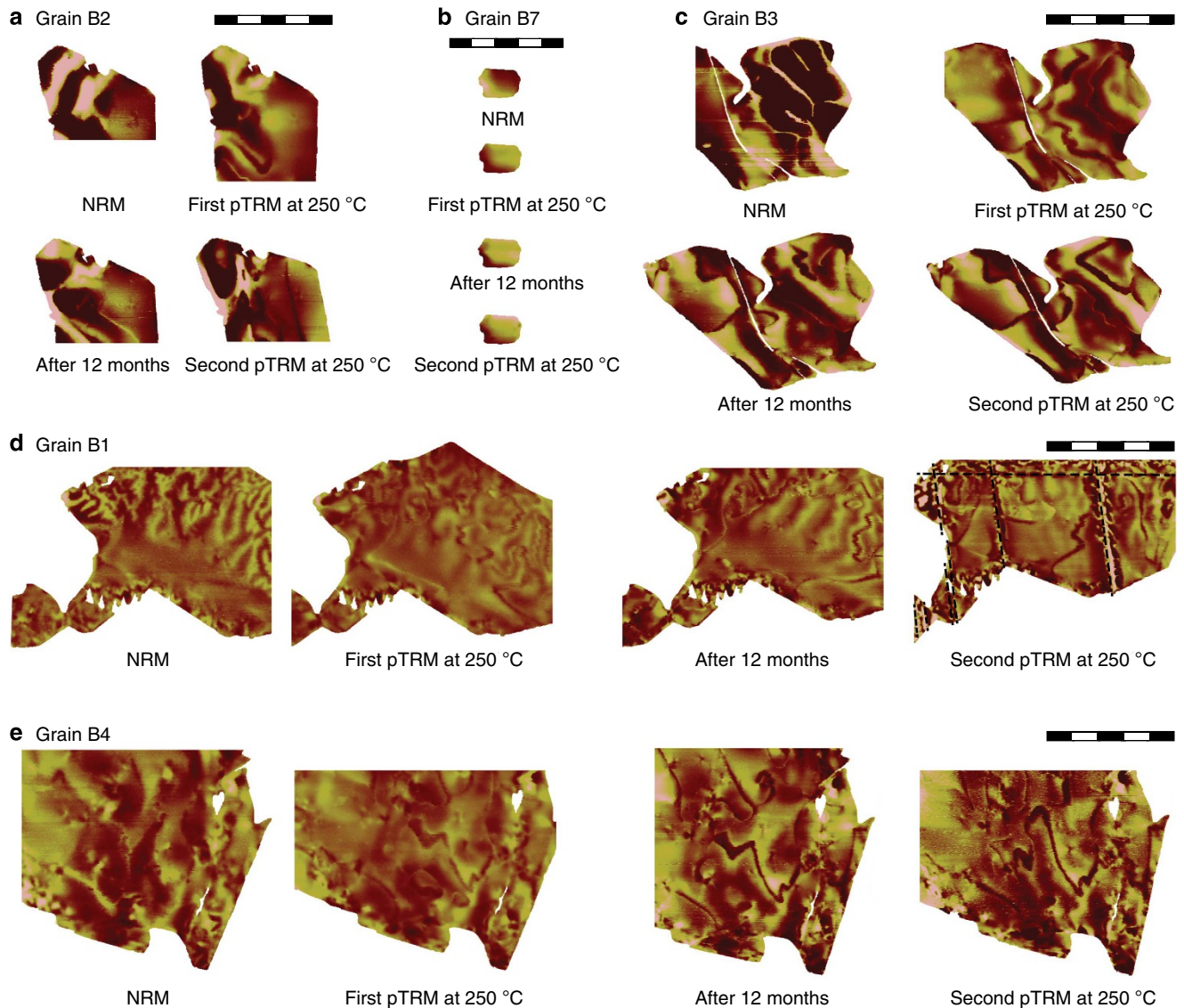
Figure 4 | Grains in the sample subjected to a pTRM at 250 °C. All scale bars are 5 μm. Four images are given per grain analysed: (1) the MFM image of the grain in its NRM state; (2) an image of the grain in its pTRM state; (3) the domain configuration after storing the samples for 1 year in a magnetic-field-free environment after the first pTRM was acquired; and (4) an image of the domain configuration after imparting a second pTRM. Except for the smallest grain analysed (B7) (b), all grains change the type of domain configuration from blocky, rectangular domains in the NRM state to curvy domains that in some grains appear as shells in their pTRM state (a, c, d, e). Furthermore, domain walls are less distinct, therefore probably wider, in the pTRM state compared with the NRM state. This is best illustrated by the right half of grain B3 (c). This new domain configuration, however, is not stable over time: after 1 year, domains become more rectangular in shape and domain walls more distinct, as visualized in the centre of grain B1 (d) and grain B4 (e). The second pTRM partly restores the curvy domains, although sample B1 was scratched (black dashed lines) in the process of imparting the second pTRM, and closure domains are evident at the scratches. The smallest grain in this study, B7 (b), shows only two domains that flip polarity in the first pTRM state; this state is stable over time and repeated by the second pTRM imparted.
