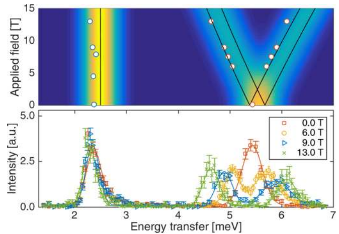
FIG. 3. The magnon energies at \mathbf{q} = (100) as a function of magnetic field along the c direction. The colors represents the calculated intensities with the black lines being the magnon positions. The circles show the center positions of the experimental data, measured at 2 K. Bottom panel shows raw data with Gaussian fits. The data were measured at RITA-II, PSI.
