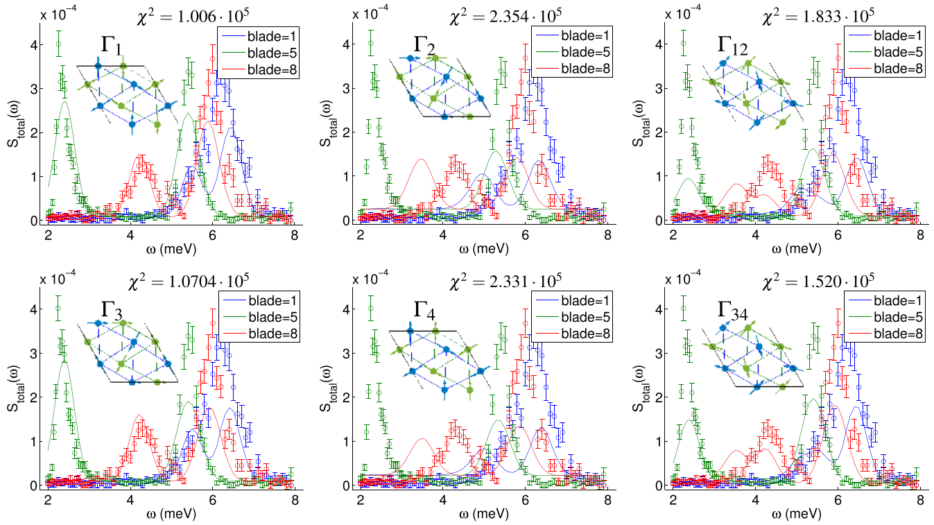
FIG. 6. Measured spectra (error bars) at T = 2 K at selected momenta in direct comparison to the full model in the ordered state for fits to calculations assuming six different ground states. The corresponding spin structures are shown in the respective insets.
