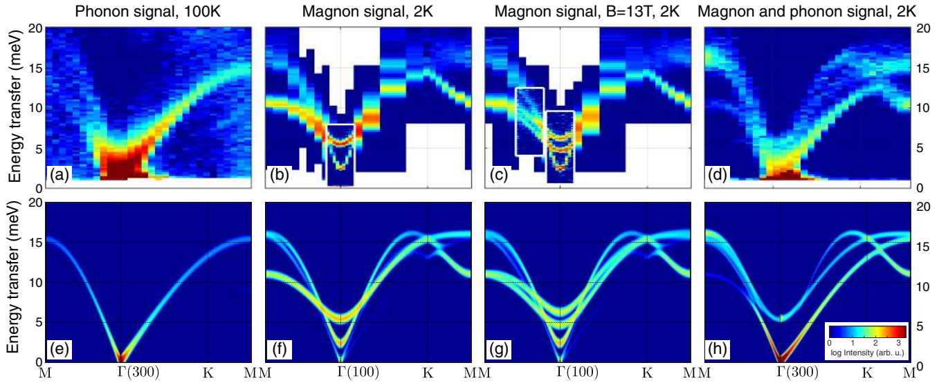
FIG. 2. Color maps of the magnon and phonon dispersions along the main symmetry directions in the (a, b) plane in reciprocal space as indicated in Fig. 1(g). Panels (a)–(d) show our experimental results. (a) and (d) are measured in BZ(300) at 100 K and 2 K, respectively. (b) and (c) are measured in BZ(100) at 2 K and with an applied magnetic field of 0 T and 13 T, respectively. The high resolution data in (b) and (c) close to \Gamma are measured at RITA-II, while the rest of the data are from EIGER; both instruments are located at PSI. Panels (e)–(h) show the theoretically calculated intensities of the dispersions at the same q values, temperatures and applied magnetic fields using the most probable magnetic ground state.
