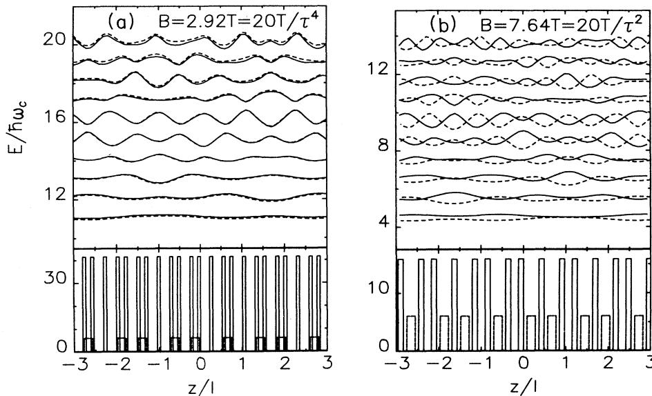
FIG. 1. (a) Magnetic energy-level structure of a quasiperiodic superlattice at B = 2.92 \text{ T} = (20 \text{ T})/\tau^4 as function the cyclotron-orbit-center coordinate (top) at zero wave vector for motion in the direction of the field. In the lower part, a section of the Fibonacci potential at the same fields. Energies are all in units of the cyclotron energy and lengths in units of the magnetic length. (b) As in (a), but for B = 7.64 \text{ T} = (20 \text{ T})/\tau^2 .
