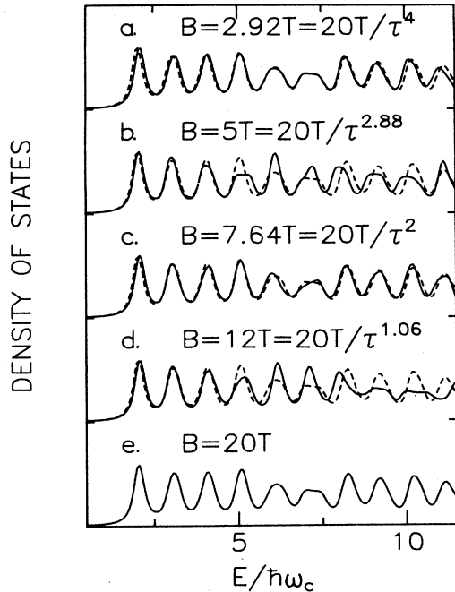
FIG. 2. Calculated density of states at zero wave vector for motion in the direction of the field. The energy scale is in units of the cyclotron energy for all curves. The zero of the energy scale for all but the lower curve is linearly shifted and aligned with the first peak. For comparison the dashed curves, all representing the results at 20 T, are drawn on the other results. Note that only for even powers of \tau is self-similarity observed.
