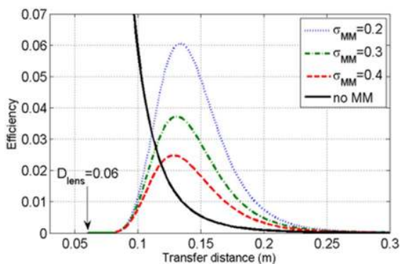
Figure 1 | Wireless power transfer efficiency of a D = 6 cm MM superlens (a layer with isotropic \mu = -1 - j\sigma ) calculated using the coupled-dipole theory 9 . The solid curve is efficiency in free space. Resistances R_{Tx} = 0.01Z_0 and R_{Rx} = 0.1Z_0 .
