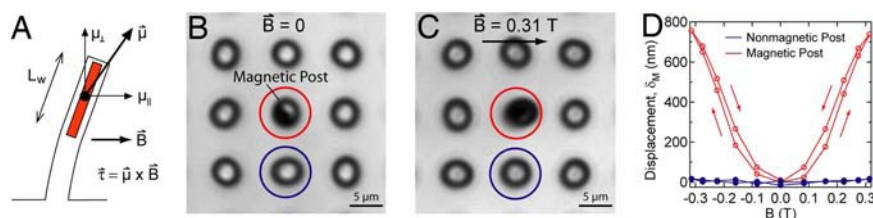
Fig. 2. Characterization of magnetic post actuation. (A) The magnetic torque, \tau , on a magnetic post of length L_w depends on the applied field, \vec{B} , the nanowire length, L_w , and dipole moment, \vec{\mu} . (B and C) Phase-contrast micrographs of a magnetic post deflected under no field and a 0.31-T field. (D) Plots of post displacement versus applied field with arrows indicating direction of driving magnetic field. Actuations caused negligible mechanical displacement in adjacent nonmagnetic post (blue curve).
