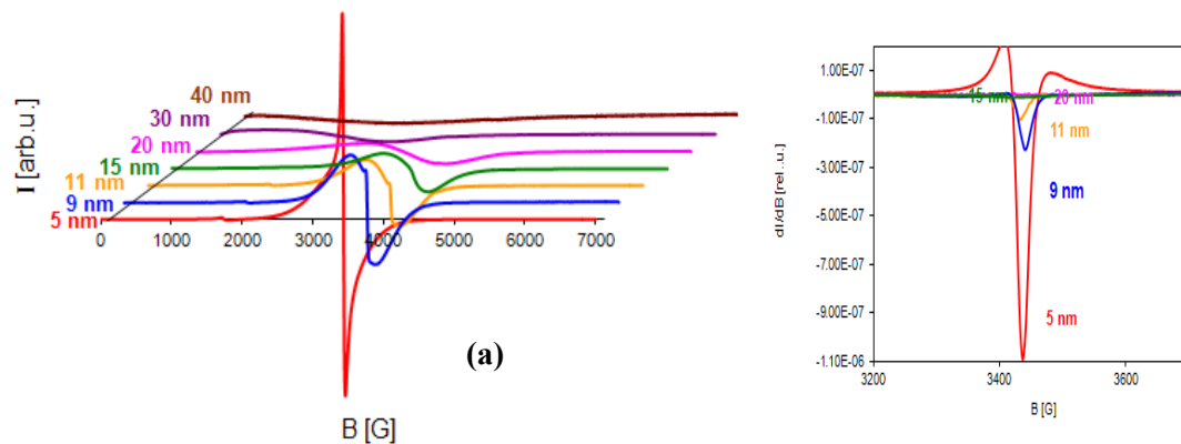
Figure 2. (a) EMR signal in ferrofluids.. (b) Derivative of EMR signal (second derivative of absorption.)
