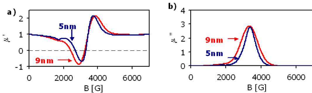
Fig. 4. Estimations of real (a) and imaginary (b) parts of permeability in dried samples with 5 nm and 9 nm particles (as indicated)
