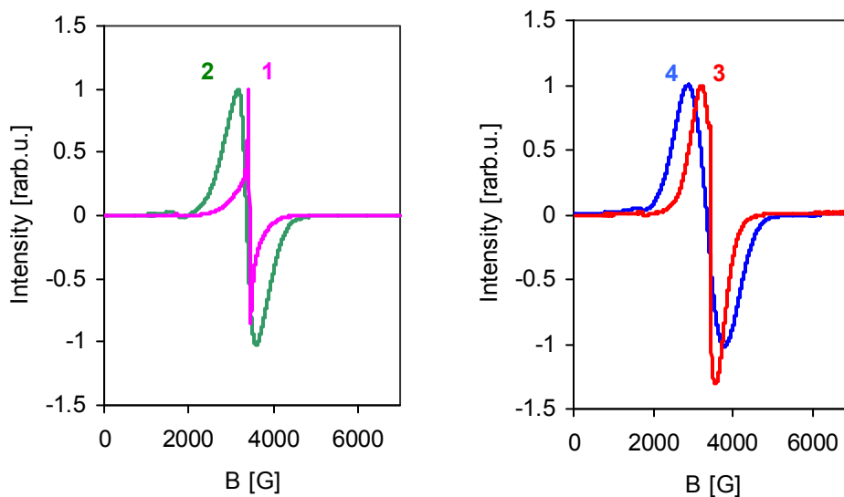
Fig. 3. EMR in diluted (Traces 1 and 3) and dried samples (2 and 4) with 5 nm nanoparticles (a) and 9 nm nanoparticles (b). The signals are normalized to maximum
