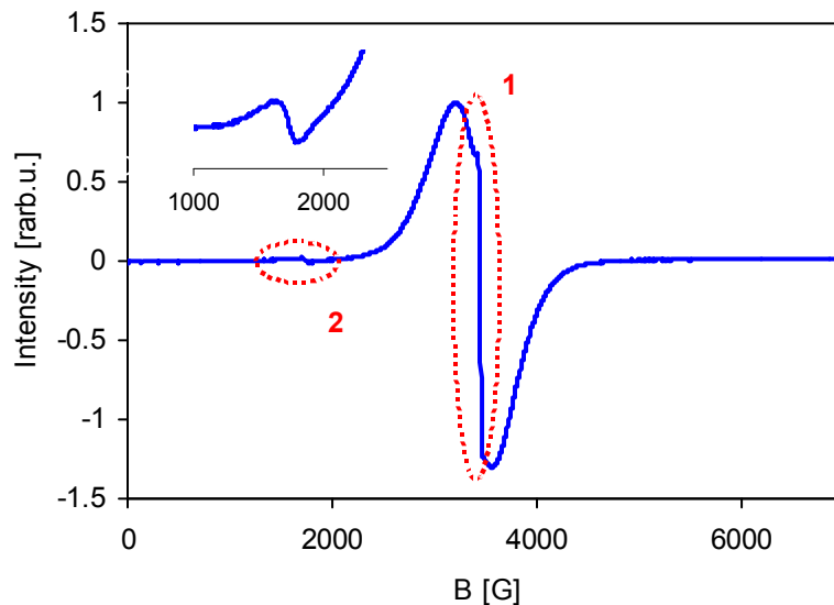
Fig. 1. Typical EMR signal in the well-diluted ferrofluid. The narrow signal at the resonance frequency (1) and half-field signal (2 and inset) are indicated.
