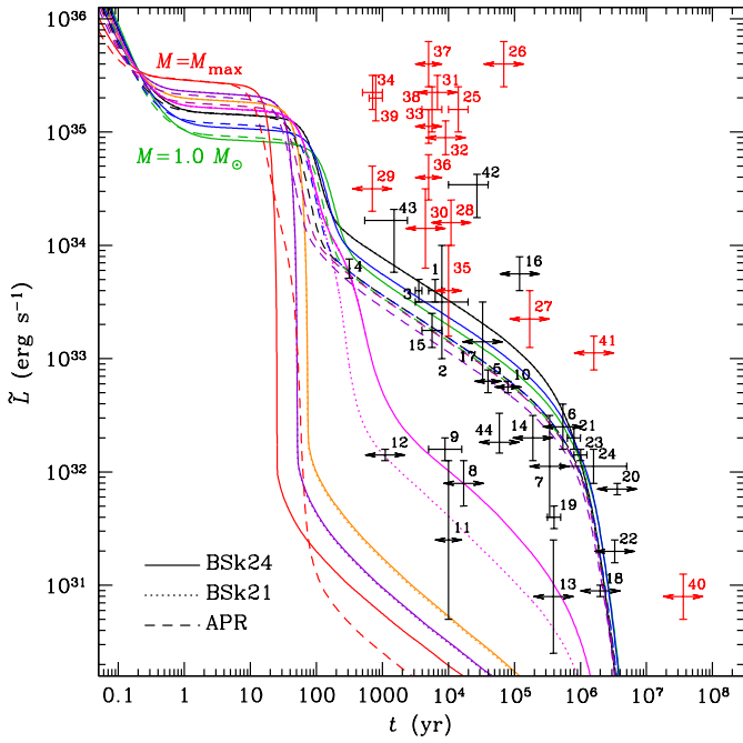
Fig. 4. Cooling curves for neutron stars with M = 1.0 (green), 1.2 (blue), 1.4 (black), 1.6 (magenta), 1.8 (orange), 2.0 M_{\odot} (violet), and the maximum mass M_{\max} (red lines), calculated using the same basic theoretical model as in Fig. 2, for the EoS models BSk24/21 (solid/dotted lines, M_{\max} = 2.28 M_{\odot} , M_{\text{DU}} = 1.596/1.587 M_{\odot} ) and APR+NV (dashed lines, M_{\max} = 2.21 M_{\odot} , M_{\text{DU}} = 2.01 M_{\odot} ) compared with observations (the same symbols as in Fig. 2).
