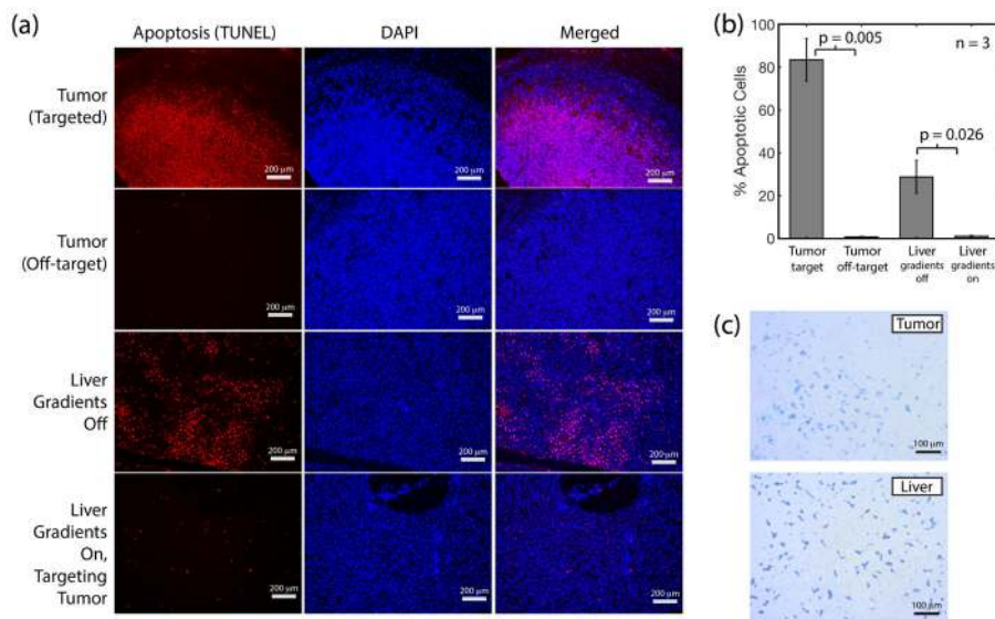
Figure 10. Histological assessment of MPI localization of thermal damage. (a) Apoptosis assay (red) and DAPI stain (blue) shows apoptosis only occurs in the targeted tumor but not in the neighboring off-target tumor, verifying localization of heat damage by the MPI gradients. The liver is also damaged when MPI gradients are turned off and uniform heating of the tumor and all other locations occurs. In contrast, no damage is observed in the liver when the MPI gradient is turned on and targeted at the tumor. (b) Statistics ( n = 3 , p -value = 0.005 with Welch's t-test) show localization of thermal damage by MPI gradients. The liver sustains damage if MPI gradients are off due to collateral heating of the SPIONs cleared to the liver. In contrast, the liver is negligibly damaged if MPI gradients are on ( p -value = 0.026). These results validate the ability of MPI gradients to localize thermal damage to the tumor while sparing the liver 1 – 2 cm away. (c) Prussian Blue stain confirms that SPIONs are successfully delivered to both the tumor and liver (clearance organ).
