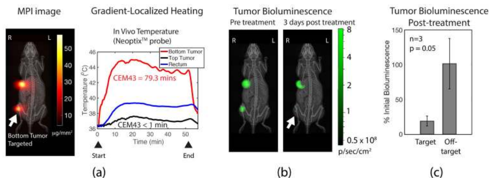
Figure 9. Experimental assessment of localized heat therapy using a bioluminescence-competent MDA-MB-231-luc xenograft model. (a) MPI image of the dual tumor MDA-MB-231-luc xenograft mice. The bottom tumor is targeted during gradient-localized heating. in vivo temperature at both tumors and the rectum measured by Neoptix™ fiber optic temperature probes. The greatest heating occurred in the targeted bottom tumor, while the upper tumor received negligible heating. The total CEM43 achieved was 79.3 minutes in the targeted bottom tumor. The core body temperature, however, was slightly elevated and likely due to the homeostatic response distributing heat from the heated bottom tumor to the rest of the body. (b) Luciferase bioluminescence activity of the tumor was measured before and after treatment. The results show a greater than 6-fold decrease in activity for the treated bottom tumor, while the untreated tumor had almost no change in bioluminescence activity. Thus, this demonstrates the utility of MPI gradients in localizing tumor therapy. (c) Statistics ( n = 3 , p -value = 0.05 with Welch's t-test) show localization of therapy to the tumor while sparing off-target sites.
