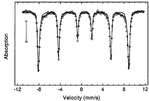
FIG. 3. Mössbauer spectrum obtained at 15 K of the as-prepared sample (circles) and of sample C1 (shown as a solid line between data points). The spectrum of the as-prepared sample is scaled by a factor 0.54 such that absorption areas of the hematite component are the same in the spectra. The vertical bar represent 2% absorption for the sample C1.
