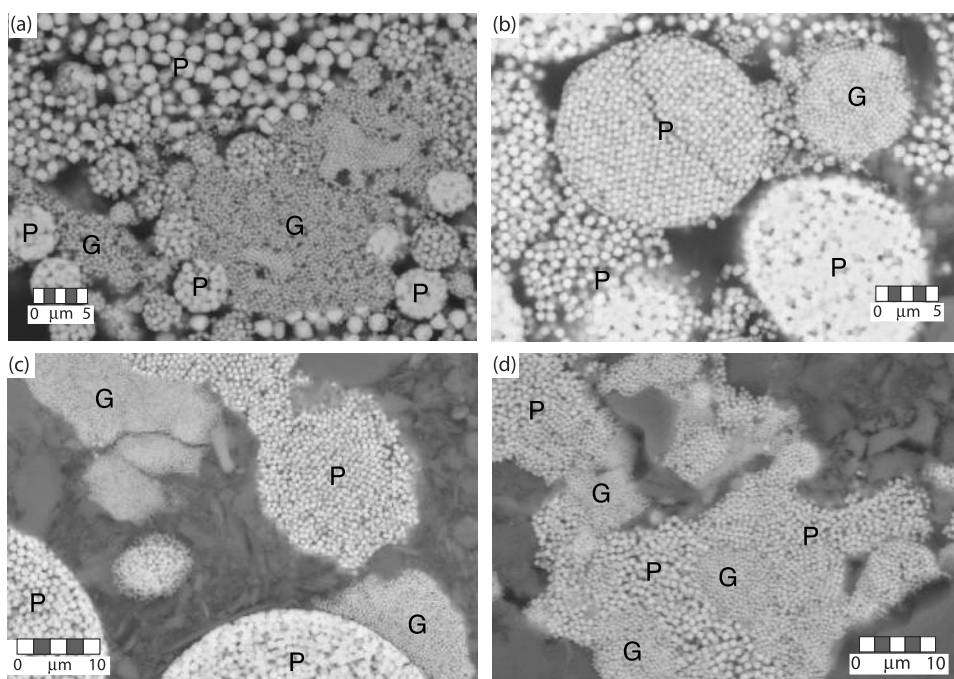
Figure 6. Backscattered electron images illustrating greigite microtextures and occurrence in sediments. (a) Aggregate of fine-grained greigite (G) filling space inside a foraminifer (Crostolo River section, Po Valley, Italy [cf. Tric et al. , 1991], sample CR07B, site 2 [Roberts et al., 2005]). (b and c) Spherical framboids of greigite (fine-grained) and pyrite (P; coarser-grained) crystals. (d) Mixed aggregate of fine-grained greigite and coarser pyrite crystals within sediment matrix (sample CR11B, site 3 [Roberts et al., 2005]). The closely packed greigite aggregates are common in diagenetically reduced sediments, which explains why FORC diagrams for sedimentary greigite routinely indicate strong magnetostatic interactions.
