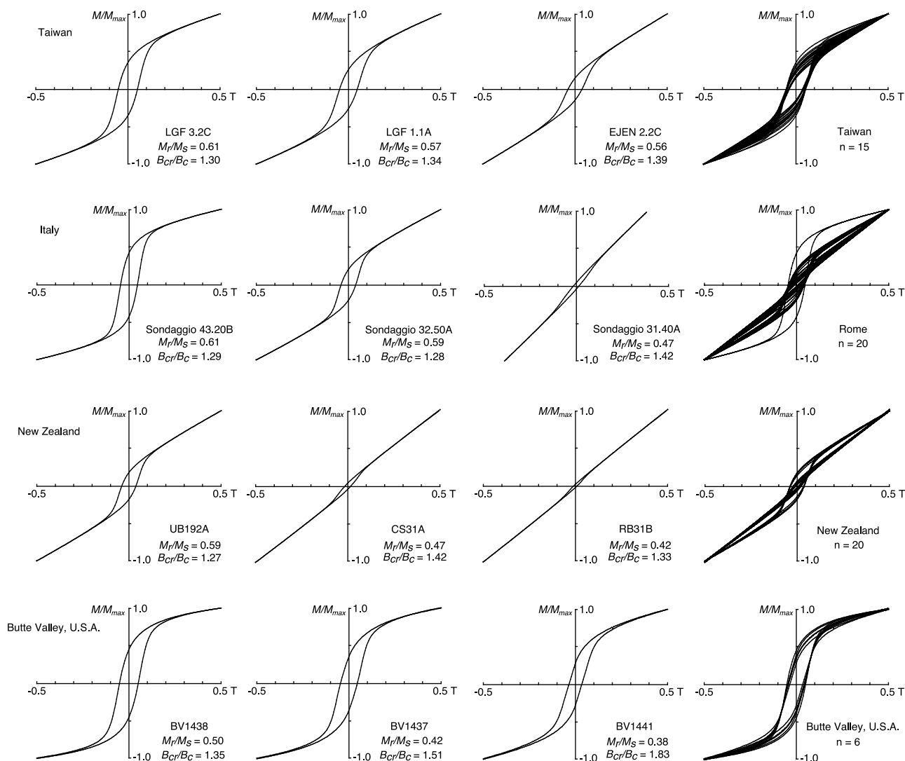
Figure 4. Magnetic hysteresis loops for greigite-bearing samples from southwestern Taiwan [Horng et al. , 1992a, 1992b]; Rome, Italy [Florindo et al. , 2007]; Marlborough, New Zealand [Roberts, 1992; Roberts and Turner, 1993]; and Butte Valley, California [Roberts et al. , 1996]. The loops in the first, second, and third columns represent the most open, intermediate, and the most closed loops, respectively, for the range of analyzed loops shown in the fourth column. Loops for samples from Taiwan and Butte Valley are consistently open. Some loops for samples from Rome are similar to the open loops from Taiwan, but there is a trend toward increasingly closed and potbellied loops. Loops for samples from New Zealand are even more closed and potbellied. Potbellied loops indicate increased importance of SP particles [Tauxe et al. , 1996] in addition to stable SD greigite. While SP particles were recognized previously [e.g., Roberts, 1995], the extent of their dominance in samples with potbellied loops was not previously recognized.
