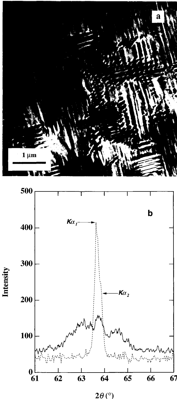
FIGURE 3. (a) Transmission electron micrograph of sample SP20 after a single high-temperature susceptibility experiment. (b) Smoothed XRD trace of the 440 reflection for sample SP20 after a single high-temperature susceptibility experiment (solid line) and the same reflection in the starting material (dashed line).
