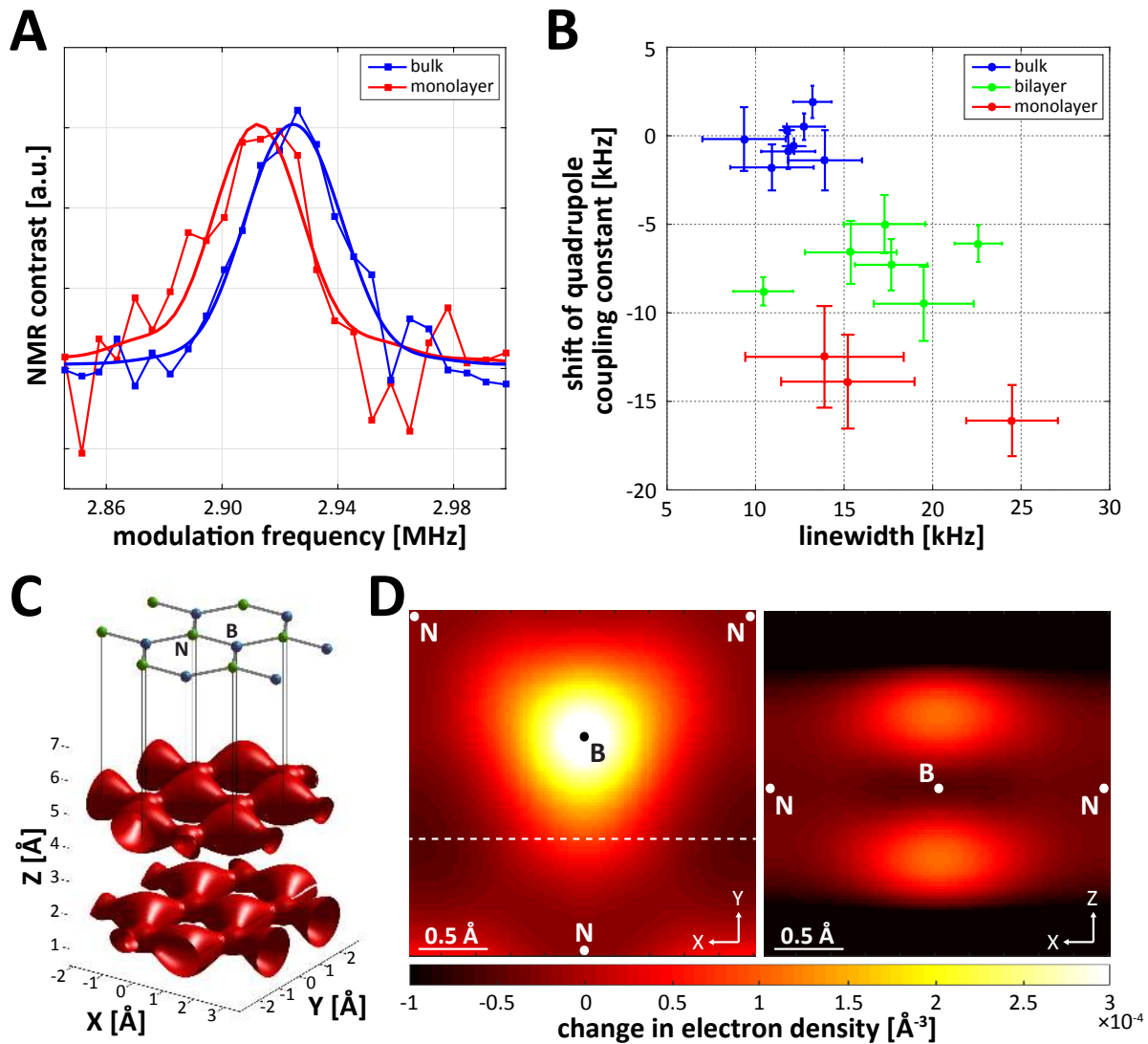
Figure 4: NQR spectroscopy of a h-BN monolayer and bilayer (A), ^{11}\text{B} NQR spectrum using XY8-187 of thick (greater than 50 nm) h-BN flake (blue) as compared to a monolayer (red). Magnetic field is aligned with respect to NV symmetry axis. Spectra have been normalized so that the resonances have the same magnitude, for comparison. The integration time for the monolayer data was approximately one day, or one hour per datapoint. (B), Values of the shift of \bar{Q} and deconvolved linewidths for several NV centers under a monolayer flake (red), a bilayer flake (green) and five bulk flakes (blue). Error bars correspond to 1-sigma uncertainties. (C), Visualization of electron density for two layers of bulk h-BN, as calculated with DFT. A single contour, corresponding to a density of \sim 1 \text{ \AA}^{-3} is shown. Boron and nitrogen sites are indicated in the schematic of atomic structure (top) (D), Left panel: visualization of the excess electron caps in the X/Y plane ( 0.8 \text{ \AA} above the atom plane). A single unit cell is shown. The image corresponds to the difference between the monolayer and bulk electron densities. Right panel: visualization of the excess electron caps in the X/Z plane (Y value indicated by dashed line in left panel). Projected positions of boron and nitrogen ions indicated.
