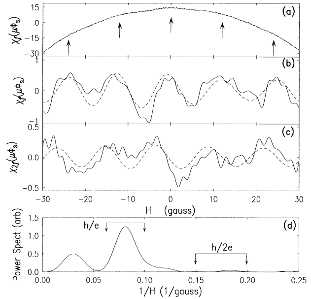
FIG. 2. The magnetic-field dependence of the amplitude of the f and 2f signals at 7.6 mK for the 1.4- \mu\text{m} \times 2.6\text{-}\mu\text{m} loop. (a) f response with no signal processing. The arrows point to the maxima of the h/e periodic signal. (b) Data of (a), with the quadratic background subtracted. (c) 2f response, after subtraction of a linear background signal. The amplitude of the 4-Hz ac drive field was 4.12 G. (d) Power spectrum for the data displayed in (b). The h/e arrows show the region, centered about the expected frequency for h/e oscillations, over which we bandpassed the data in (b) and (c) to produce the dashed curves. The region where an h/2e signal is expected to appear based upon the inside and outside area of the sample is also shown. The data in (b) and (c) have been digitally filtered to eliminate high-frequency contributions above 0.50 \text{ G}^{-1} .
