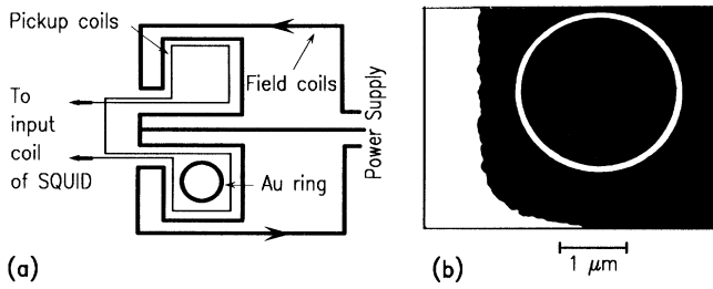
FIG. 1. (a) Schematic diagram of the pickup coil chip, illustrating the counterwound Nb pickup coils and the on-chip magnetic-field coils. (b) Micrograph of the 2.4- \mu\text{m} -diam Au ring in one corner of the 9- \mu\text{m} -inner-diam Nb pickup coil. The loop linewidth is 90 nm and the thickness is 60 nm.
