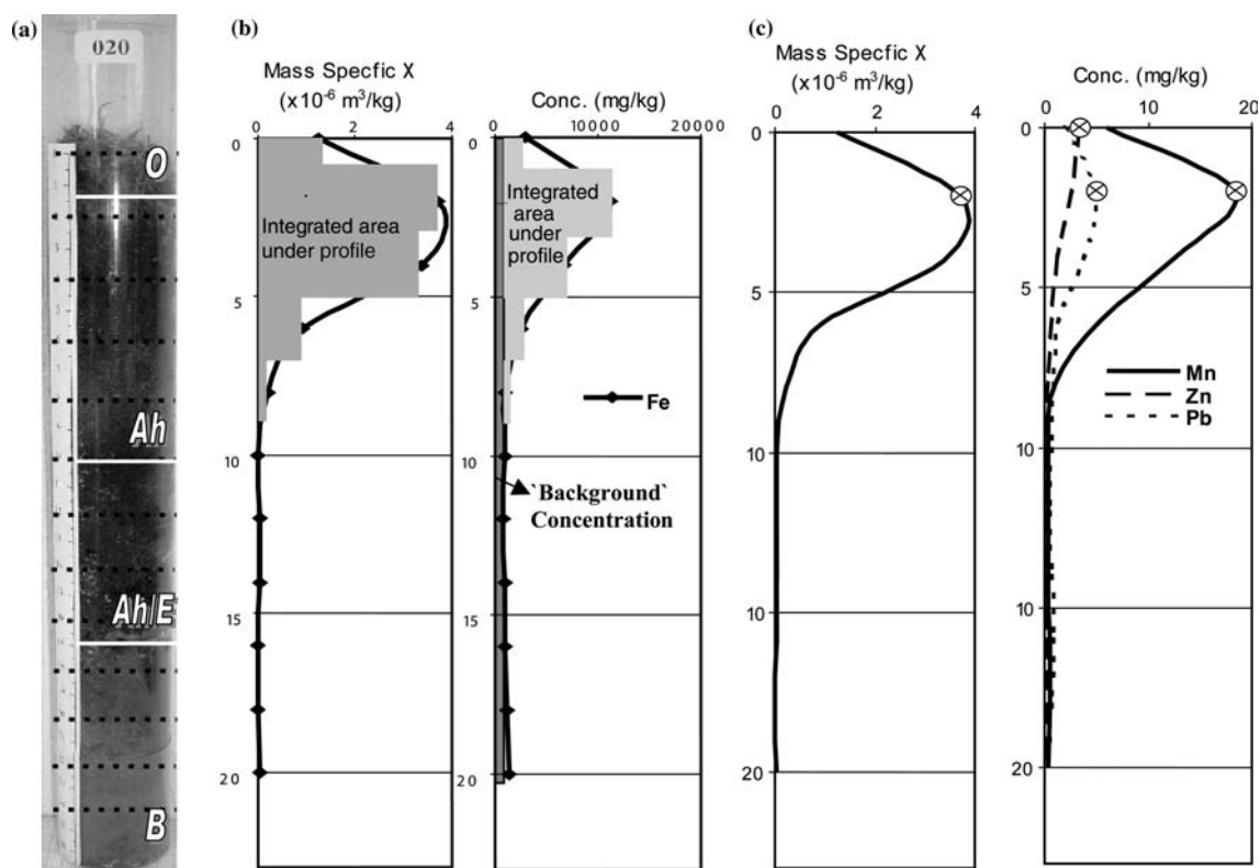
Fig. 1 a Photo of Core 20, depicting subsamples referred to as Individual sample - sample analysis ; b KLY-2 magnetic susceptibility profiles (individual samples measured with KLY-2) and heavy metal profiles showing integrated area and 'background' area; c KLY-2 and heavy metal profiles showing measured peak value, marked with
