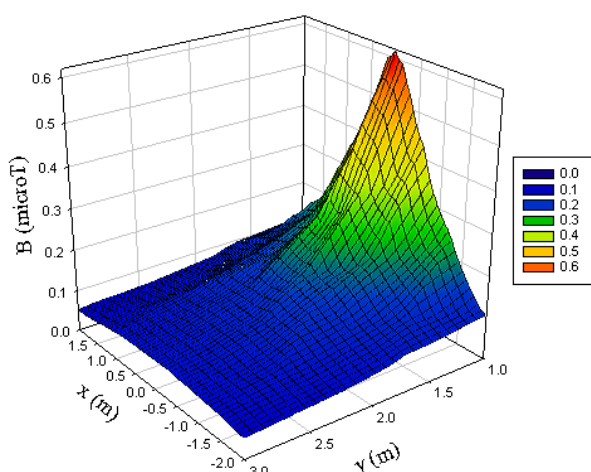
Figure 6. Magnetic field distribution with a shield of 200 mm-length arms.
