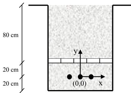
Figure 1. Ditch and position of the underground conductors.
