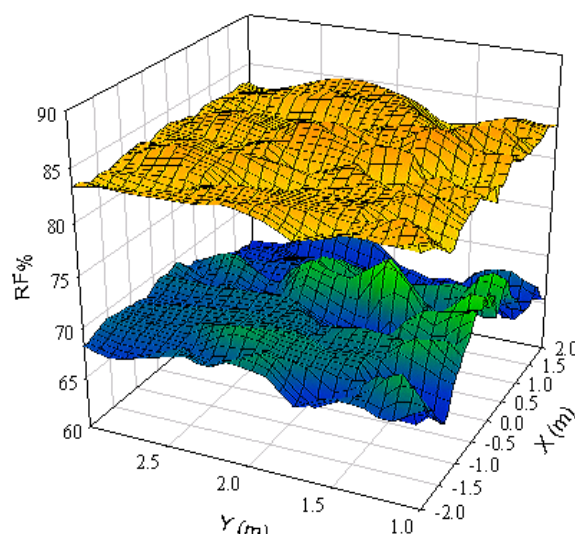
Figure 7. Comparison of the magnetic field reducing factor for two different shields geometries (up: l = 0 mm, bottom: l = 200 mm).
