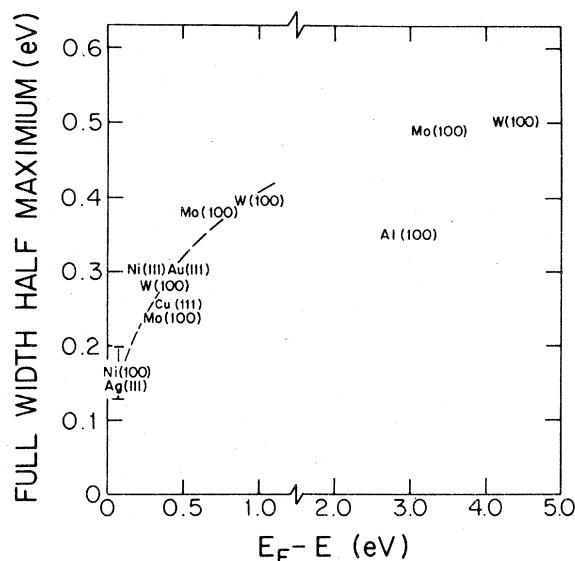
FIG. 7. Full width at half maximum (FWHM) of surface states on metals. Ag(111), Au(111), and Cu(111), Ref. 8; W(100) and Mo(100), Ref. 5; Al(100), Ref. 31; and Ni(111) Ref. 12.
