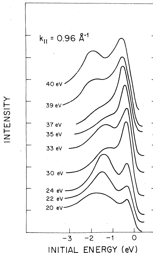
FIG. 3. Photon energy sweep for fixed k_{\parallel} in [11] direction. s polarized light in the "even" geometry used in Fig. 2.
