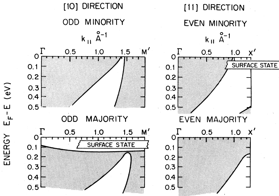
FIG. 6. Projection of the bulk bands onto the two symmetry directions of the surface Brillouin zone. The odd majority and minority bands are projected onto the [10] direction ( \Gamma to M' ). The even bands are projected onto the [11] direction ( \Gamma to X' ).
