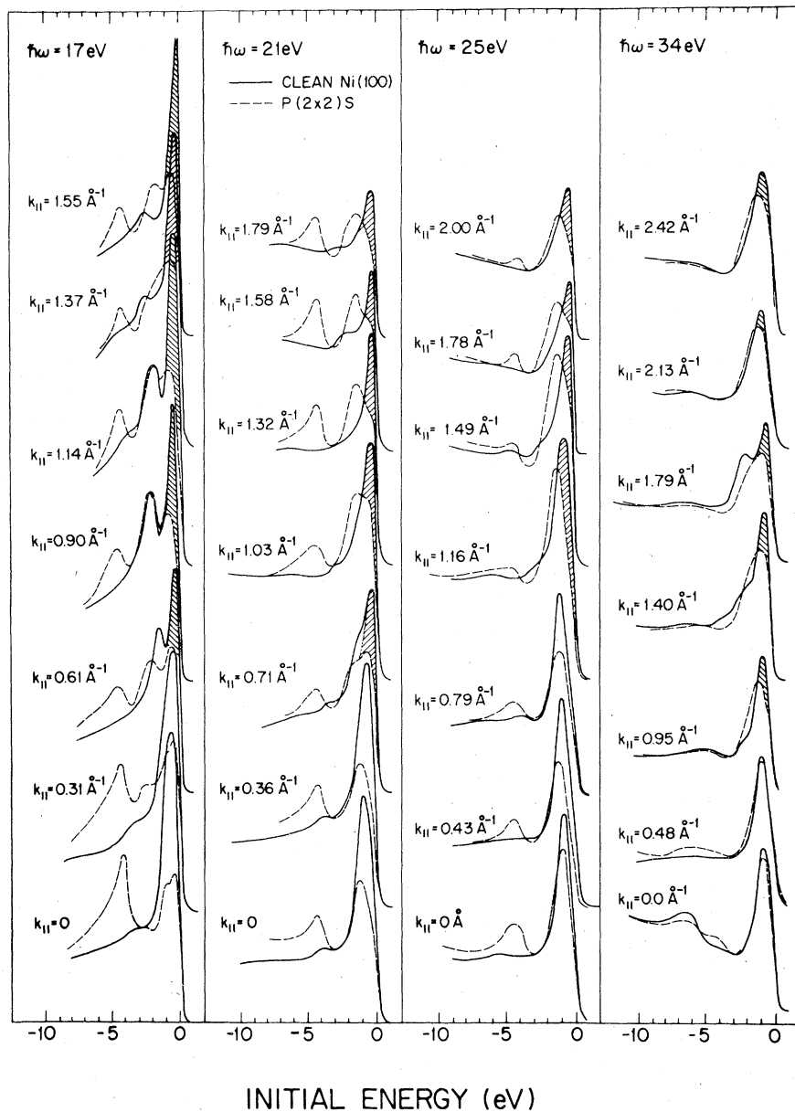
FIG. 4. Comparison of photoelectron spectra of clean Ni and Ni with p(2 \times 2)S overlayer for four photon energies and several values of k_{||} . The measurement geometry is the "even plus odd" geometry of Fig. 2, with k_{||} along the [10] direction.
