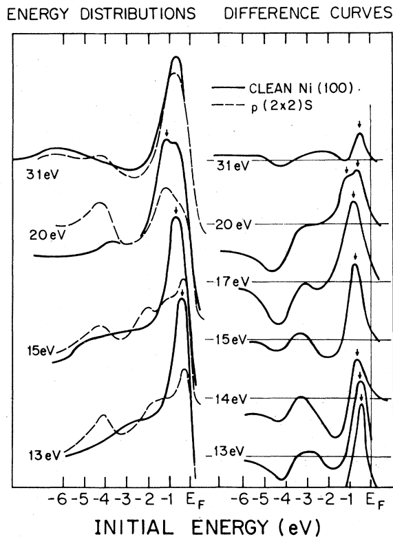
FIG. 8. Photoelectron spectra for normal emission for Ni(100), using p -polarized light. The curves on the right are difference spectra [clean p(2 \times 2)S ].
