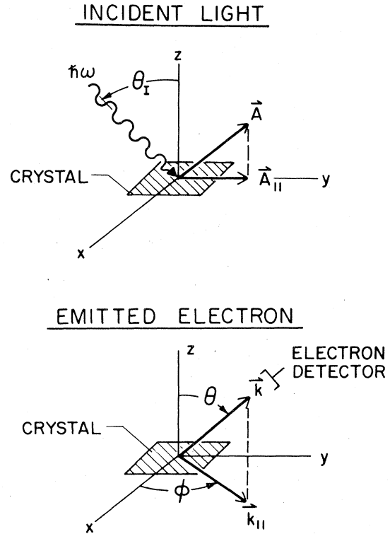
FIG. 1. Schematic drawing of the geometry of the angle-resolved photoemission measurements.
