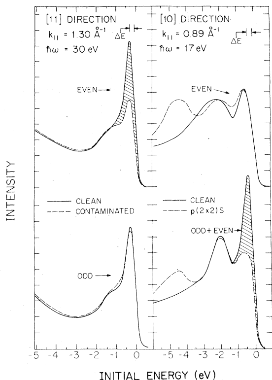
FIG. 2. Angle-resolved photoelectron spectra from Ni(100). The spectra on the left are taken at \hbar\omega = 30 eV using s -polarized light [ \theta_I = 0^\circ ]. The collection angle is \theta = 30^\circ [ k_{\parallel} = 1.30 \text{ \AA}^{-1} ]. \vec{A} is always in [11] direction. The curves marked odd (even) are for collection perpendicular (parallel) to a \vec{A} . The spectra on the right are in the [10] direction for \hbar\omega = 17 eV, \theta = 30^\circ [ k_{\parallel} = 0.89 \text{ \AA}^{-1} ] and p -polarized light [ \theta_I = 45^\circ ]. The curves marked "even" are for a collection geometry in the plane of incidence ( \varphi = 90^\circ ). The "odd plus even" denotes collection perpendicular to the plane of incidence.
