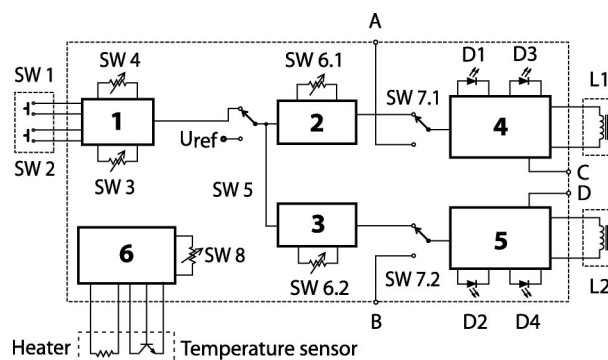
FIG. 4. Block diagram of the control unit. 1—Pulse generator; 2, 3—preamplifiers; 4, 5—voltage/current converters and power amplifiers; 6—temperature control unit; L1, L2—coils; SW1—pulse train trigger; SW2—manual pulse trigger; SW3—pulse length adjustment; SW4—time between pulses adjustment; SW5—pulse/continuous magnetic field switch; SW6.1 and SW6.2—current adjustment; SW7.1 and SW7.2—external/internal pulse switch; SW8—temperature adjustment; A, B—external pulse inputs; C, D—current monitor outputs; U_{\text{ref}} —internal dc reference for continuous field. Indicators (light): D1, D2—pulse monitor LED; D3, D4—overload LED.
