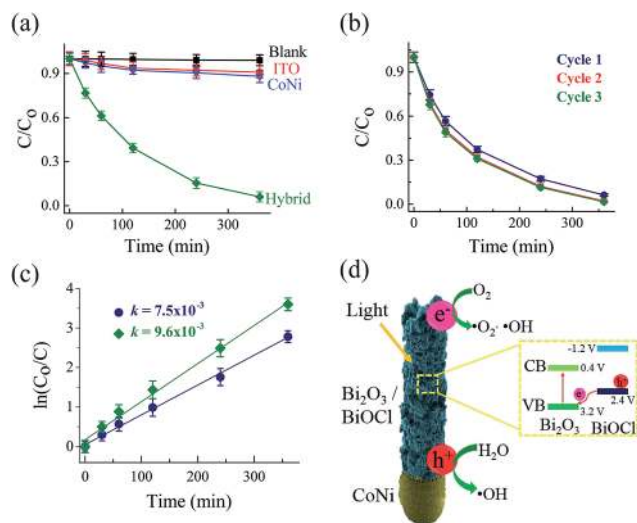
Fig. 3 Photocatalytic degradation of hybrid micropillars. (a) Photocatalytic degradation curves of blank, ITO covered glass slide, free-standing \text{CoNi} , and hybrid structures upon light irradiation; (b) plot showing degradation curve results for three consecutive runs for the same sample; (c) linear fit log plot of the degradation curve for cycle 1 and 3 showing an enhanced k value for cycle 3; (d) photocatalytic degradation scheme of hybrid micropillars showing the formation of electron-hole pairs and how they degrade organic pollutants.
