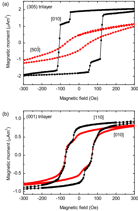
FIG. 4. (Color online) Magnetization measurements on (a) (305)-oriented and (b) (001)-oriented F/S/F trilayers. The bottom and top F layers are 50 and 150 nm, respectively; the S layer is 30 nm. Measurements are taken at temperatures slightly above T_c of the superconductor. The magnetic field directions are indicated in the figure. The (305)-oriented trilayers show uniaxial magnetic anisotropy. The magnetization loop for the (001)-oriented trilayers shows somewhat sharper features when measured along the [110] direction than along the [010] direction, in accordance with literature (Ref. 27).
