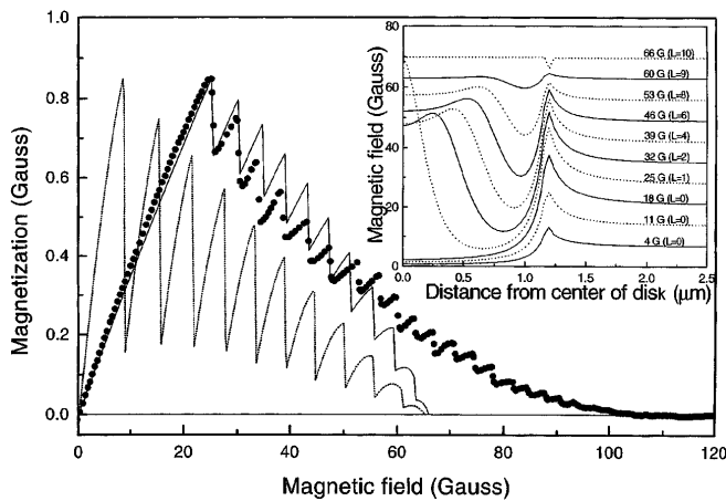
FIG. 3. The same as Fig. 1 for a disk of radius R = 1.2 \mu\text{m} and thickness d = 0.15 \mu\text{m} . In the inset we show the field distribution in the plane through the center of the disk for different values of the external magnetic field. Far away from the center of the disk the magnetic field equals the external magnetic field.
