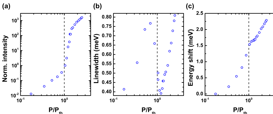
FIG. 3. (a) Input-output curve and (b) power dependent linewidth trace of the ground state emission. Slightly above threshold, the linewidth narrows down to 0.391\ \text{meV} (smaller than for low excitation powers). (c) Energy peak position versus excitation power. All the values are extracted from the momentum-space spectra by integrating around k_{||} = 0 with k_{||} = \pm 0.15\ \frac{1}{\mu\text{m}} .
