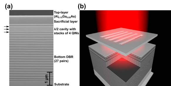
FIG. 1. (a) SEM image of the epitaxial structure which is utilized for the device fabrication. It consists of a \frac{\lambda}{2} -cavity with three stacks of 4 QWs. The position of the QWs is indicated by arrows. (b) Schematic sketch of the structure after etching and fabrication steps.
