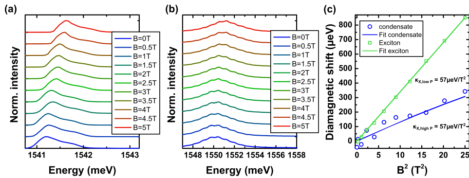
FIG. 4. Line spectra from the momentum-space images for the different magnetic fields from B = 0 T to B = 5 T at an excitation power of P = 1.4P_{th} for (a) the polariton condensate and (b) the uncoupled QW exciton. (c) Comparison between the diamagnetic shift of the bare quantum well exciton (green squares) and the diamagnetic shift of the polariton condensate (blue dots).
