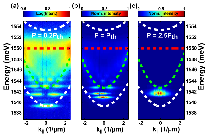
FIG. 2. (a)–(c) Energy-momentum dispersions of a 5\ \mu\text{m} large high index contrast grating structure at a detuning of \delta = -7\ \text{meV} . The white dashed lines are indicating the lower and upper polaritons, the red dashed line the exciton, and the green dashed one the photon energy. (a) Well below the non-linearity threshold at P = 0.2P_{th} , the zero-dimensional resonances are clearly visible confirming the 3D confinement of the structure. (b) At the threshold P = P_{th} , the ground state energy is slightly blueshifted and becomes more and more intensive. Above threshold (c) at P = 2.5P_{th} only the ground state is observable. The emission occurs well below the photon energy (green dashed line) indicating that strong coupling is preserved.
