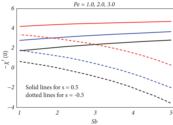
FIGURE 7: Variation of reduced density number of the motile microorganisms -\chi'(0) with bioconvection parameters.
