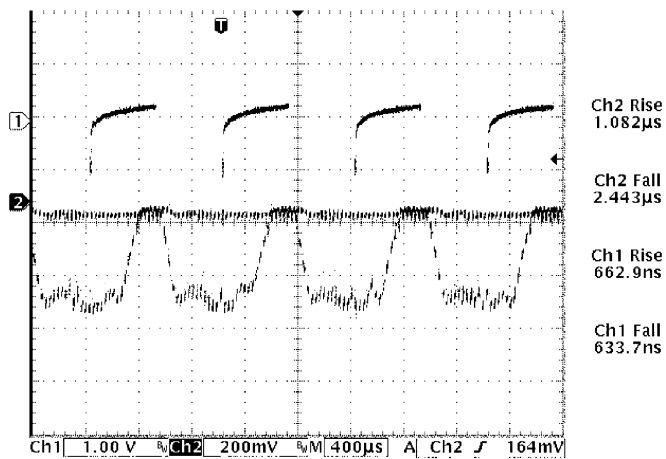
Fig. 4. Measured external applied voltage (channel 1) and the switching of the optical signal (channel 2) waveforms.
