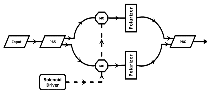
Fig. 3. Schematic of the proposed switch with polarizers in both paths.
