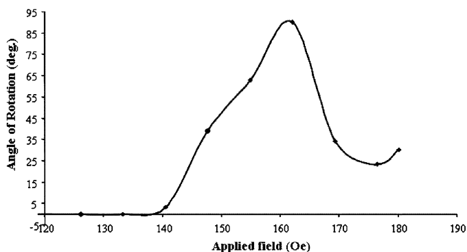
Fig. 2. Measured Faraday rotation for the MO rotator clearly shows nonlinear behavior.
