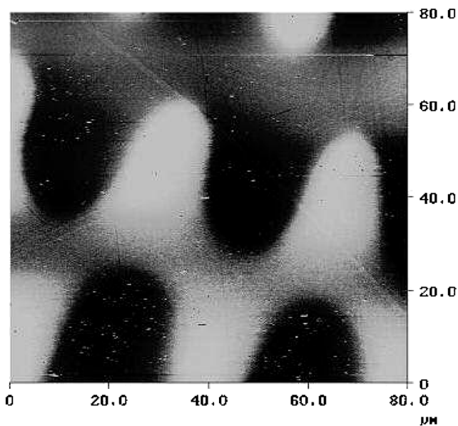
Fig. 1. Magnetic force microscope image of the domains that measure about 20 \mu\text{m} .
