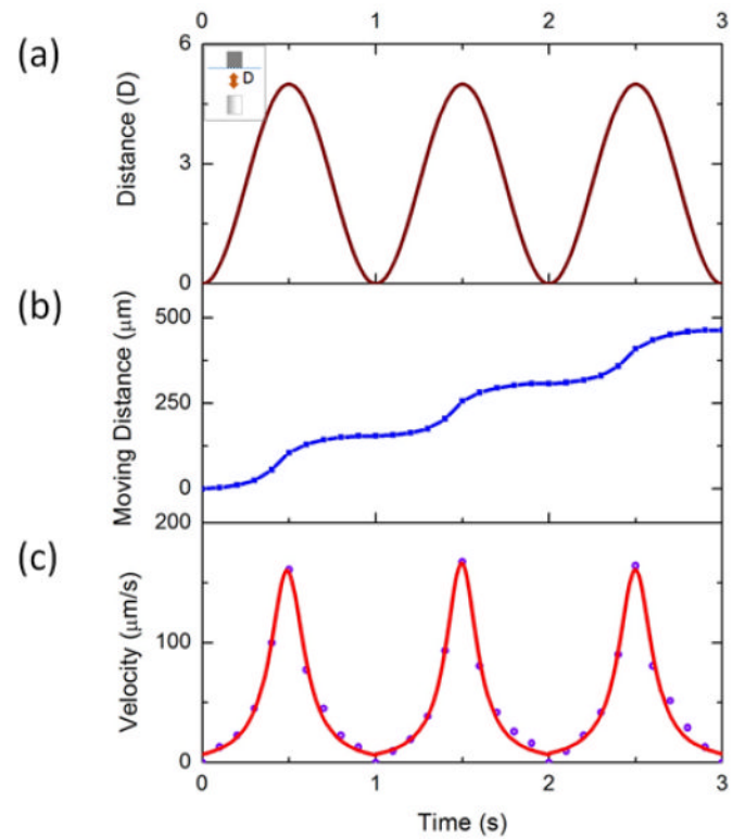
FIGURE 2. Method for generating flow patterns. (a) The distance between magnet and magnetoactive sponge as a function of time. (b) Representative plot of particle movement vs. time at 1Hz frequency. (c) Particle velocity profile (solid points) and its fitting curve.
