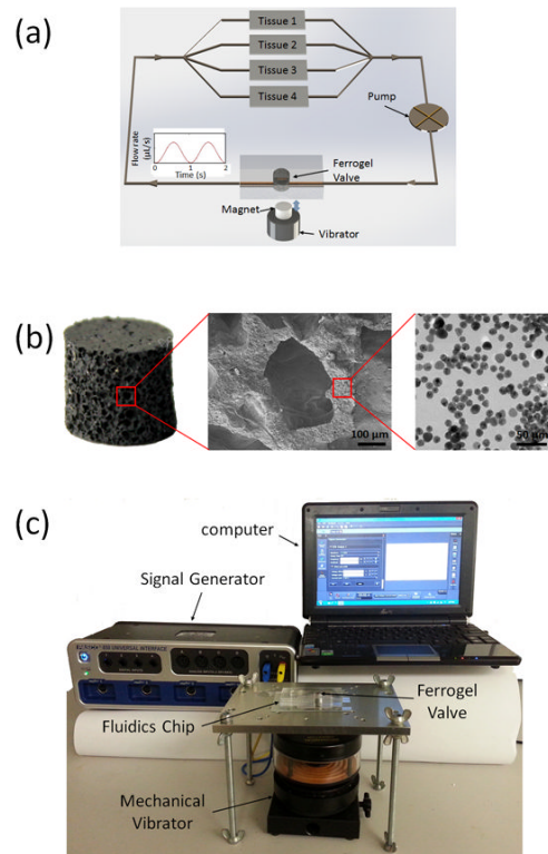
FIGURE 1. (a) The schematic diagram of the configuration of fluidic system. (b) The photograph of porous sponge (left), the SEM image of pore (middle) and the TEM image of dispersed iron powder (right). (c) A photograph of the flow control system.
