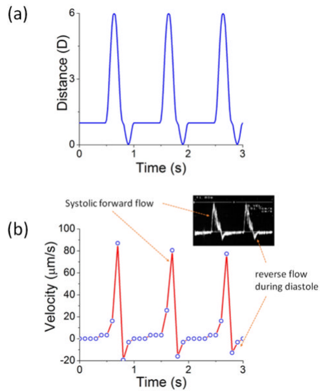
FIGURE 5. Generation of physiological flow pattern. (a) Prescribed distance between the magnet and magnetoactive sponge as a function of time. (b) Measured physiological flow pattern. (Inset: ultrasound scan of typical biphasic blood waveform at common femoral artery 38 )
