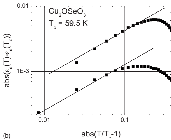
FIG. 6. (a) The temperature dependence of the dielectric constant. The solid line is a fit. (b) Critical behavior of the magnetic contribution to the dielectric constant.
