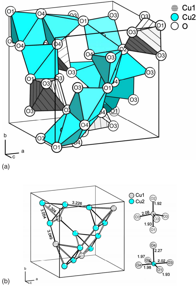
FIG. 1. (Color online) (a) Polyhedral representation of the crystal structure of \text{Cu}_2\text{OSeO}_3 with \text{SeO}_3\text{lp} polyhedrons omitted. (b) Connectivity of the Cu ions and local coordination environments of Cu1 and Cu2. The labeling of atoms is consistent with that used in Table I.
