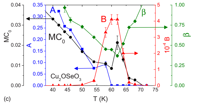
FIG. 7. (Color online) (a) Magnetocapacitance in low applied fields illustrating the anomaly that occurs at the metamagnetic transition. The inset shows the magnetic H - T phase diagram. (b) Fits to the field dependence of the magnetocapacitance (see text) at temperatures below ( T = 25 K) and at the magnetic transition ( T = 60 K). (c) Temperature evolution of the fitting constants MC_0 , A , B , and \beta (see text).
