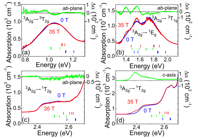
FIG. 4. (Color online) (a,b) Close-up view of the {}^3A_{2g} \rightarrow {}^3T_{2g} , {}^3A_{2g} \rightarrow {}^1E_g , and {}^3A_{2g} \rightarrow {}^3T_{1g} absorption bands at 0 and 35 T along with the full field absorption difference in the ab -plane. (c,d) Close-up views of the {}^3A_{2g} \rightarrow {}^1T_{2g} excitation in the ab -plane and c -directions. The red, green, and blue hash marks indicate calculated d -to- d excitations for Ni1, Ni2, and Ni3.
