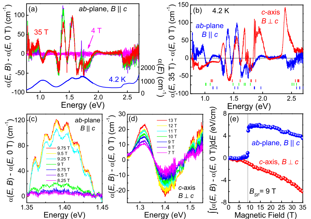
FIG. 3. (Color online) Absorption difference spectra, \Delta\alpha = [\alpha(E, B) - \alpha(E, B = 0 \text{ T})] , of \text{Ni}_3\text{TeO}_6 in the (a) ab -plane for B \parallel c at selected fields up to 35 T: (pink 4 T, purple 10 T, green 20 T, red 35 T). The 4.2 K absolute absorption spectrum is included for comparison (on the bottom, in blue). (b) Full field (35 T) absorption difference spectra taken in the ab -plane and along the c -direction. Red, green, and blue vertical lines indicate the predicted d -to- d excitations. (c,d) Absorption difference spectra in the ab -plane ( B \parallel c ) and c -direction ( B \perp c ) at selected fields around the spin-flop transition. (e) Integrated absorption difference of the data in panels (c) and (d).
