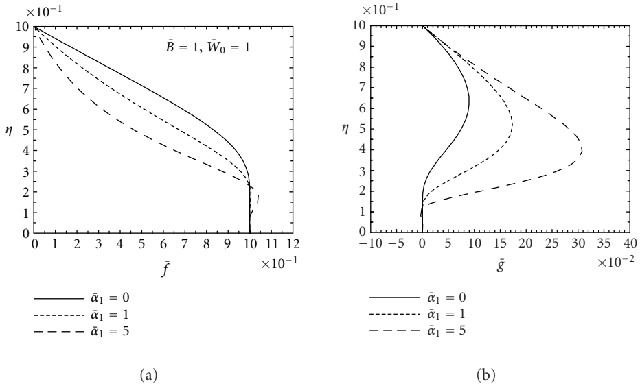
Figure 4.4. Profiles of dimensionless translational velocities \bar{f} (panel a) and \bar{g} (panel b) for a non-Newtonian fluid with various coefficients of the second-grade terms \bar{\alpha}_1 = 0 (a Newtonian fluid), 1, 5. The third-grade and fourth-grade terms are neglected ( \bar{\beta}_i = 0, i = 1, 2, 3; \bar{\gamma}_i = 0, i = 1, 3, 4, 5 ).
