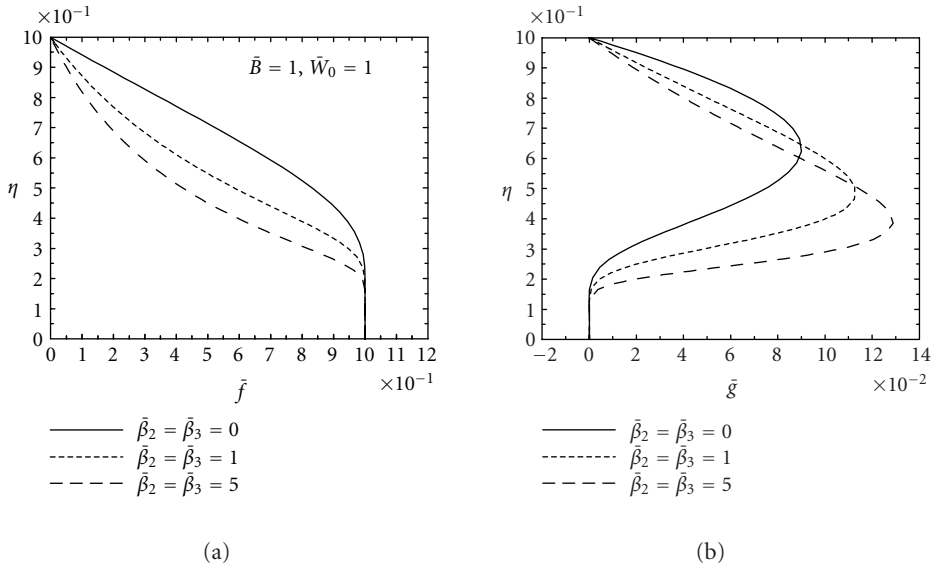
Figure 4.5. Profiles of dimensionless translational velocities \bar{f} (panel a) and \bar{g} (panel b) for a non-Newtonian fluid with various coefficients of the third-grade terms \bar{\beta}_{2,3} = 0 (a Newtonian fluid), 1, 5. The second-grade and fourth-grade terms are neglected ( \bar{\alpha}_1 = 0; \bar{\gamma}_i = 0, i = 1, 3, 4, 5 ).
