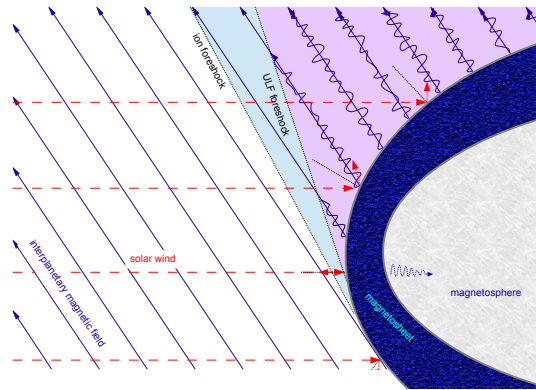
Fig. 35 Sketch of upstream waves generated in the quasi-parallel foreshock region by solar wind protons backscattered from the Earth's bow shock.
