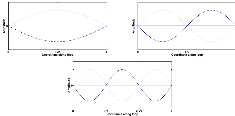
Fig. 26 Displacements of the plasma in the global mode (top left), its second harmonic (top right), and third harmonic (bottom) for a loop of length L . The black line shows the position of the undisturbed loop and the red dotted and blue dashed lines indicate the extrema of displacement, corresponding to different phases of the oscillation.
