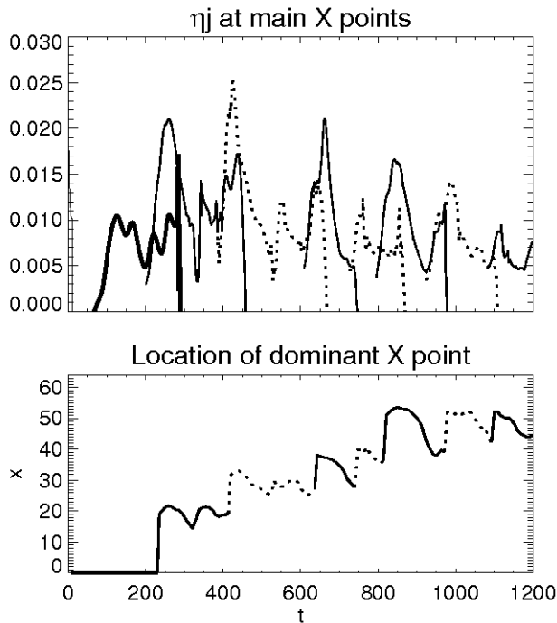
Fig. 45 Upper: Electric field at the main X-points (reconnection rate) vs. time. Bottom: Location of the dominant X-point. Distances and time are expressed in a halfwidth of the current sheet and Alfvén cross time, respectively. (From Kliem et al. 2000).
