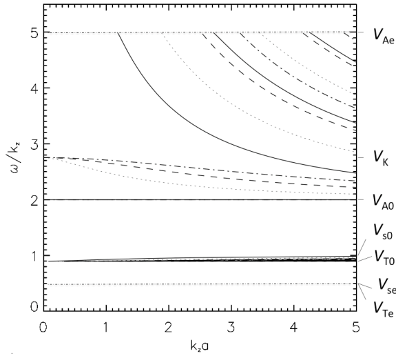
Fig. 16 Phase speeds \omega/k_z of MHD modes of a field-aligned plasma cylinder as a function of the longitudinal wave number k_z for the parameters V_{A0} = 2V_{s0} , V_{Ae} = 5V_{s0} , V_{se} = 0.5V_{s0} , V_{s0} = 1 . The horizontal dash-dotted lines indicate the characteristic speeds. The solid horizontal line shows the torsional Alfvén waves. The solid curves are solutions for m = 0 , the dotted lines for m = 1 , the dashed lines m = 2 and the dash-dotted for m = 3 modes. Figure adapted from Nakariakov and Verwichte (2005).
