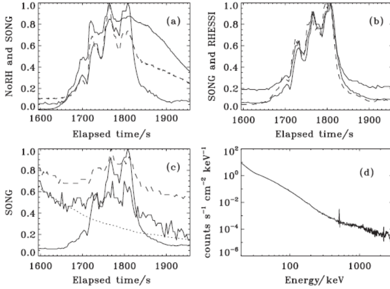
Fig. 43 Time development of a typical solar flare with QPPs of the microwave, hard X-ray and gamma-ray emission. (a) Intensity of 17 GHz (solid) and 34 GHz (dashed) emission recorded with the Nobeyama Radioheliograph, and hard X-ray emission at 42–80 keV (thick) recorded with CORONAS-F/SONG; (b) 80–225 keV (thin) recorded with CORONAS-F/SONG, and 50–100 keV (dashed), and 100–300 keV (thick) recorded with RHESSI; (c) 80–225 keV (thick), 225–750 keV (dashed), and 2–6 MeV (thin solid) recorded with CORONAS-F/SONG; the dashed curve shows the averaged 2–6 MeV light curve from previous orbits. The elapsed time is measured from 00:00 UT on 1 January 2005. (d) Photon energy spectrum integrated between 00:28 UT and 00:32 UT obtained with RHESSI. The light curves are normalised to their maximum values. (From Nakariakov et al. 2010b).
