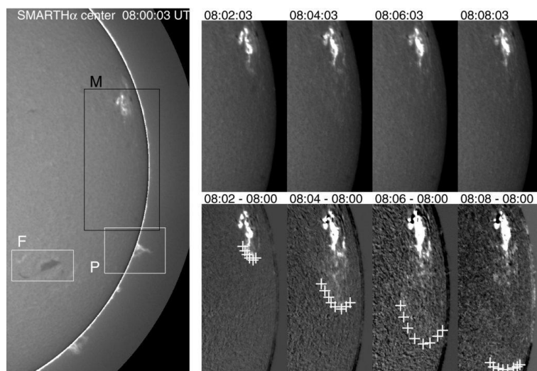
Fig. 4 Example of a Moreton wave observed with the Solar Activity Research Telescope (SMART) http://www.hida.kyoto-u.ac.jp/SMART/ . The region “M” in the left panel outlines the region of interest from where a sequence of H \alpha images are given in normal intensity (top-right panel) and running difference intensity (top-bottom panel). The Moreton wave front is marked by white plus signs. (From Asai et al. 2012).
