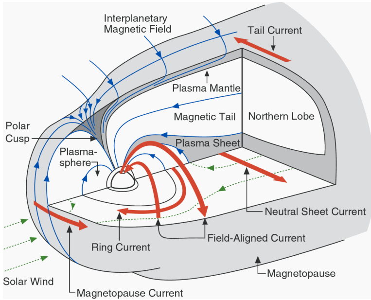
Fig. 2 A sketch of the Earth's magnetosphere structure.
