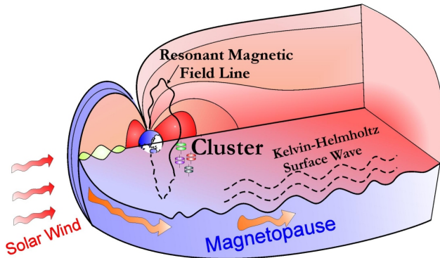
Fig. 34 Schematic illustration of Kelvin–Helmholtz instability onset at the magnetosphere flanks. The excited surface modes are coupled with Alfvén field line oscillations.
