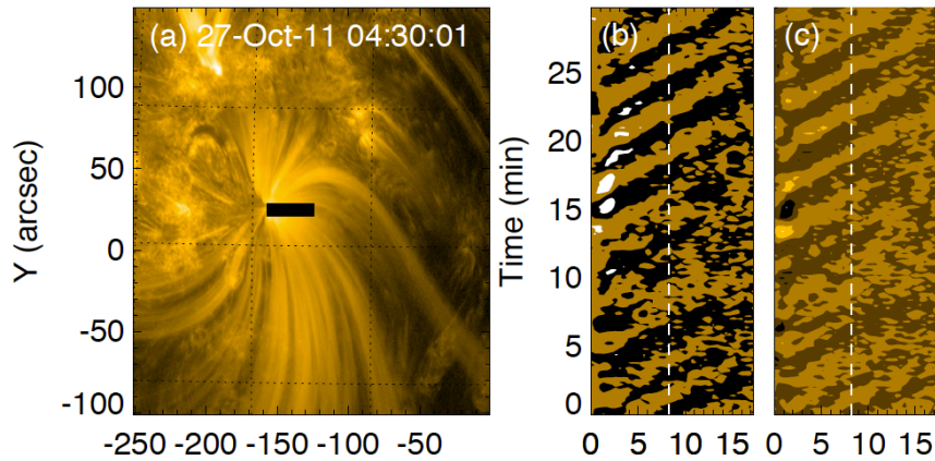
Fig. 29 Example of a propagating quasi-periodic longitudinal oscillation in a coronal plasma fan. a) SDO/AIA 171Å image of active region NOAA 11,330 observed on 27 October 2011 at 04:30:01 UT. A cut that was taken to make the time–distance plot is indicated with a black bar. b) Time–distance plot of the running difference, made along the cut. It covers about 10 cycles of the propagating features. c) The same time–distance plot but made with the background-subtraction method. The diagonal stripes in panels b and c indicate the outwardly propagating waves of the EUV intensity. (From Yuan and Nakariakov 2012).
