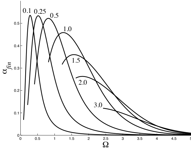
Fig. 20 Frequency dependence of the conversion coefficient \alpha(\Omega) , numerically calculated for a modelled profile \rho(z) , for different values of normalised wave vector K .
