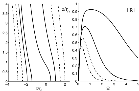
Fig. 11 Left-hand panel: 2D magnetic field configuration. Right-hand panel: Reflection coefficients of poloidal Alfvén modes propagating along the curved field lines. The curves |R(\Omega)| and the corresponding field lines are shown by the same type of line: heavy, light, dashed, and dashed-and-dotted, for diverging field lines.
