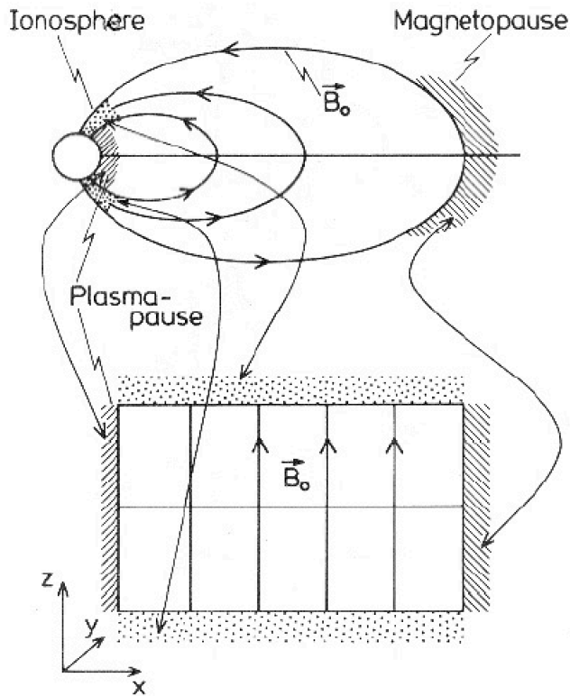
Fig. 18 Schematic illustration of the correspondence between the magnetospheric box model and realistic magnetosphere. (From Glassmeier et al. 1999).
