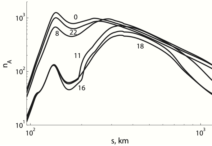
Fig. 13 Profiles of the Alfvénic refractive index n_A(s) in the mid-latitude ionosphere for various UT. The upper set of curves (UT=0, 8, 22) correspond to daytime hours, the lower set of curves (UT=11,16,18) correspond to nighttime hours.
