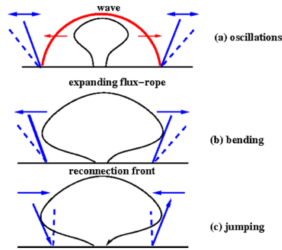
Fig. 7 Response of coronal structures (blue) to different drivers: a) oscillation from the propagation of a wave (red), which surrounds the CME flux-rope (black), b) an expanding CME flux rope pushes outwardly the structures causing bending, c) the expanding CME magnetically reconnects with the structure, which undergoes an inward jumping. (From Patsourakos and Vourlidas 2012b).
