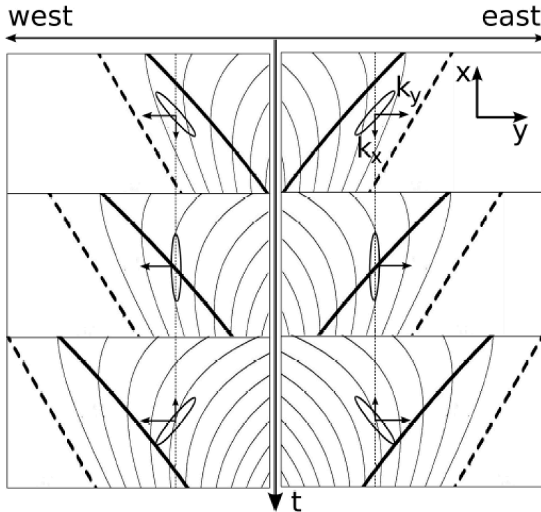
Fig. 37 Polarisation ellipses of the wave excited by the moving cloud at different time instants. Dashed lines represent the drifting source. The bold line corresponds to k_x = 0 (purely poloidal polarisation of the wave). The right and left parts of the figure correspond to electrons and ions, respectively. Thin lines represent the lines of the constant phase. (From Zolotukhina et al. 2008).
