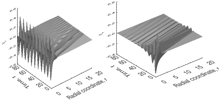
Fig. 15 Variation of the radial velocity in the standing sausage mode of a plasma cylinder, in the trapped (left panel) and leaky (right panel) regimes. (From Nakariakov et al. 2012).
