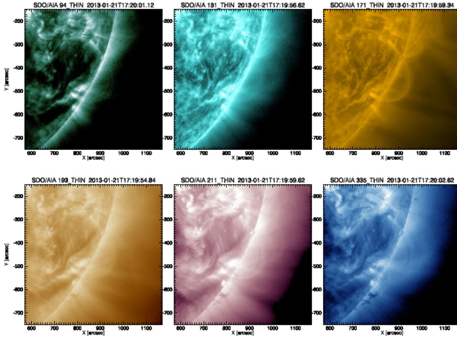
Fig. 1 A typical active region of the solar corona, situated at the solar limb and observed at six EUV wavebands of SDO/AIA. Colours in each panel are artificial, with the brightest pixels corresponding to the biggest number of EUV photons of the prescribed wavelength and hence to the denser plasma of the selected temperature.
