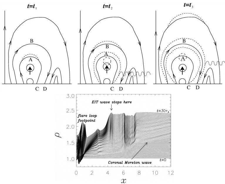
Fig. 6 Upper panels: Mechanism for the formation of global coronal waves. From Chen et al. (2002). Bottom panel: Evolution of the density profiles that initially show the propagation of a coronal Moreton waves from the flare loop footpoint, and then a trailing global coronal (EIT) wave stopping in the vicinity of a small active regions. (From Chen et al. 2005).
