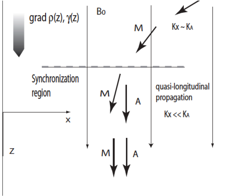
Fig. 19 Schematic illustration of the model of a plasma with a longitudinally non-uniform density \rho(z) . The arrows show the wave vectors of fast magnetoacoustic (M) and Alfvén (A) waves.
