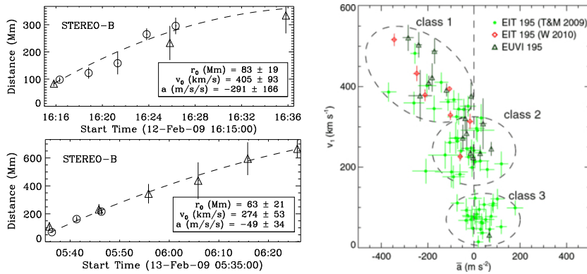
Fig. 5 Left: Plots of distance versus time of the propagating fronts for two EUV waves observed by STEREO-B. Initial speeds inferred by fitting analysis range between 250–400 \text{km s}^{-1} , and deceleration of the order of (-290) – (-50) \text{m s}^{-2} . From Long et al. (2011). Right: initial speeds versus acceleration for a large number of EUV events detected with SoHO/EIT and STEREO/EUVI. (From Warmuth and Mann 2011).
