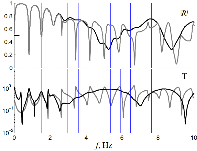
Fig. 41 Reflection R(f) and transmission T(f) coefficients for Alfvén waves with the wave numbers k_{\perp} = 10^{-3} \text{ km}^{-1} (dark line) and k_{\perp} = 10^{-2} \text{ km}^{-1} (grey line), interacting with the nightside ionosphere at mid-latitude ( I = 58.6^{\circ} ).
