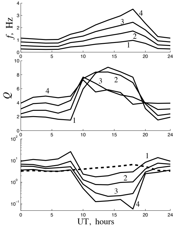
Fig. 14 Diurnal variations of the eigenfrequencies (upper panel) and Q-factors (middle panel) for the IAR harmonics ( n = 1-4 ). Bottom panel: The height-integrated Joule dissipation J = (1/2) \int_0^H \sigma_P |e_1|^2 dz (solid line) and energy flux into the magnetosphere (dashed line).
