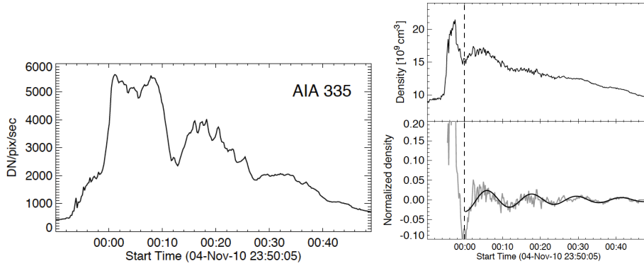
Fig. 28 Example of a standing longitudinal oscillation in a hot coronal loop, observed simultaneously in the EUV and microwave bands. Left: Time profile of maximum counts obtained at the AIA 335 Å channel in a flare loop. Right: Time profile of the electron number density derived by electron temperature and the temperature brightness at 17 GHz (top panel), and a best fitting of the detrended and normalised profile with an exponentially decaying harmonic curve (bottom panel). The vertical dashed line shows the instant of time after which the microwave emission is free-free. (From Kim et al. 2012).
