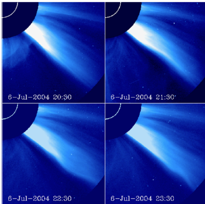
Fig. 30 Transverse motion of a coronal streamer stalk, as an aftermath of the CME impact, seen in the snapshots of coronal images taken in the white light during an artificial eclipse. The white circle in the top-left corner of the images indicates the solar limb. The wavy displacement propagating outwards at the Southern slope of the bright streamer is the transverse waves. (From Chen et al. 2010).
