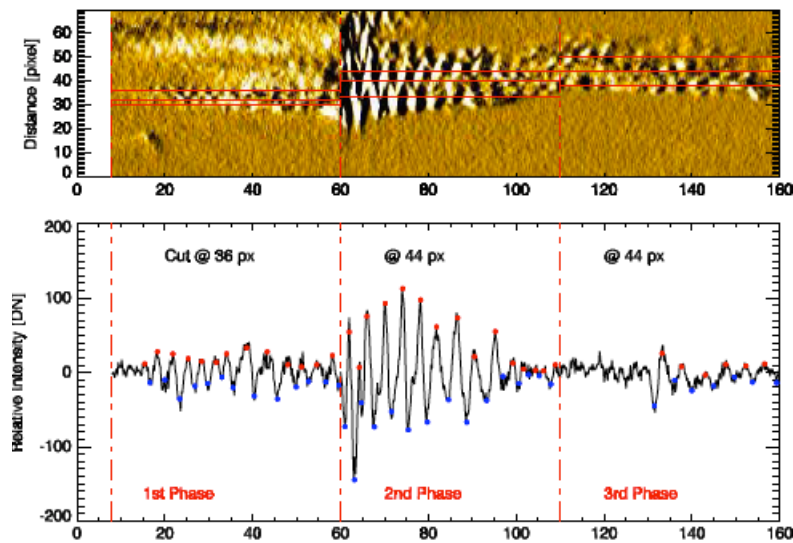
Fig. 25 Kink oscillations of a coronal loop. The top panel shows the time-distance plot made for a slit across the loop near its top. The periodic transverse displacements are clearly seen. The bottom panel shows the zoomed parts of the time distance maps: the red and blue bullet are the maxima and minima positions. The 1st and 3rd phases correspond to the decay-less low-amplitude oscillations, while the 2nd phase to the large amplitude decaying oscillations excited by a CME. (From Nisticò et al. 2013).
