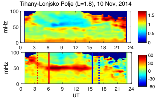
Fig. 21 The dynamic gradient method technique: the spectral transfer function G(f) (upper panel) and phase delay \Delta\psi(f) (bottom panel).
