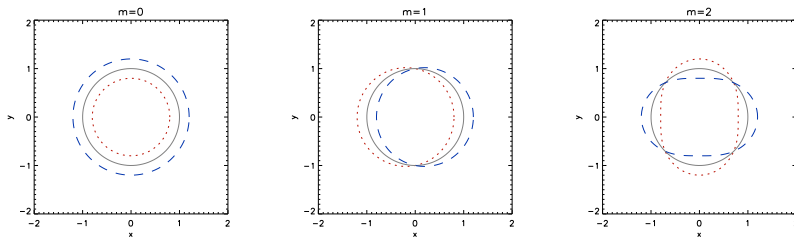
Fig. 17 Diagrams showing the structure of m = 0 (sausage) modes (left panel), m = 1 (kink) modes (middle panel), and m = 2 (fluting) modes (right panel). The solid line is the equilibrium position of the flux tube, and the dotted and dashed lines two extreme phases.
