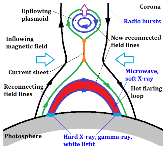
Fig. 42 Schematic sketch of the standard model of a solar flare.
