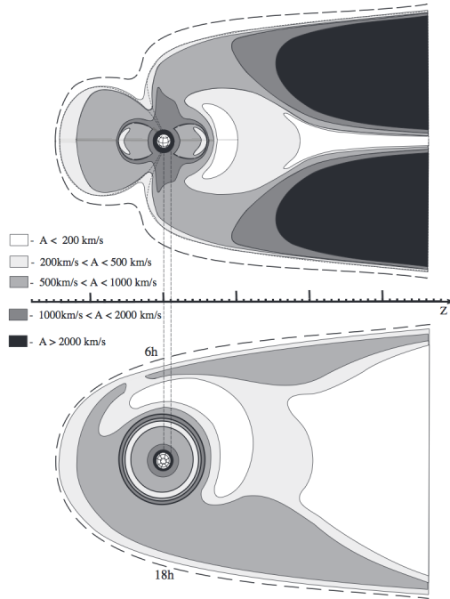
Fig. 9 A sketch of Alfvén speed distribution in the meridional (top panel) and equatorial (bottom panel) sections of the magnetosphere. Areas with different values of the Alfvén speed ( A = V_A ) are shown by varying shades of grey. (From Mazur and Leonovich 2006).
