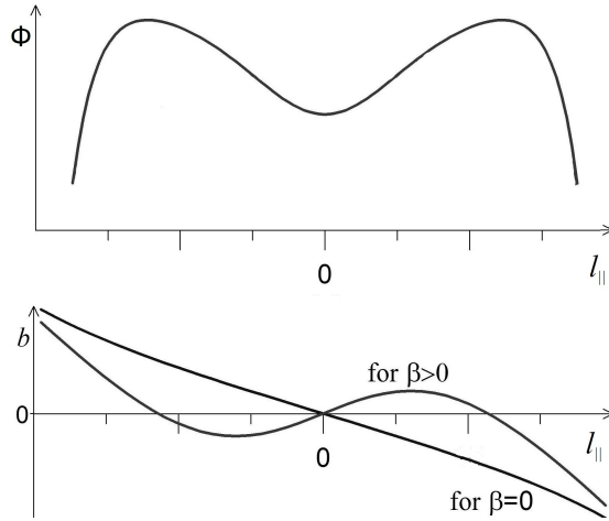
Fig. 12 Field-aligned structure of the fundamental harmonic in the vicinity of the magnetospheric equatorial plane ( s = 0 ). Shown are the wave potential \Phi(s) ( \beta > 0 case) and magnetic field b_1(s) ( \beta = 0 and \beta > 0 cases). (From Mager et al. 2009).
