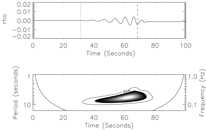
Fig. 31 Numerical simulation of an impulsively generated fast magnetoacoustic wave train propagating along a coronal loop with a density contrast ratio of 5.0 and profile steepness power index equal to 8. Upper panel: the characteristic time signature of the wave train. Lower panel: wavelet transform analysis of the signal, demonstrating the characteristic “crazy” tadpole wavelet signature. (From Nakariakov et al. 2004b).
