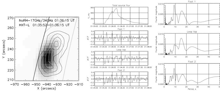
Fig. 27 Left: Radio images of an oscillating flaring loop, made at 34 GHz (filled pixels) and 17 GHz (dotted contour curves). The black contour shows the positioning of the 13.9–22.7 keV hard X-ray sources. The solid line indicates the solar limb. The dotted curves show the heliographic coordinate grid. Centre: The time profiles of the total signal, the modulation depth of the gyrosynchrotron signal at 17 GHz from the Southern leg, the loop top, and the Northern leg of the loop. Left: Fourier power spectra of the modulation depth signals. (From Melnikov et al. 2005).
